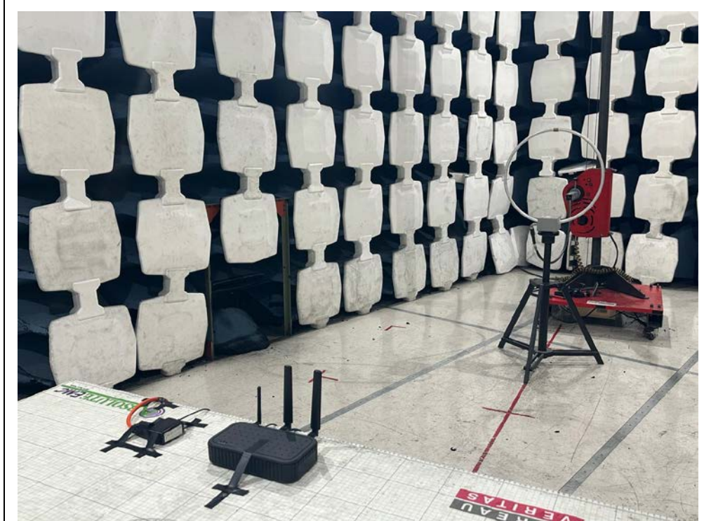
9k-30MHz Rear (H4P3-TWC)
