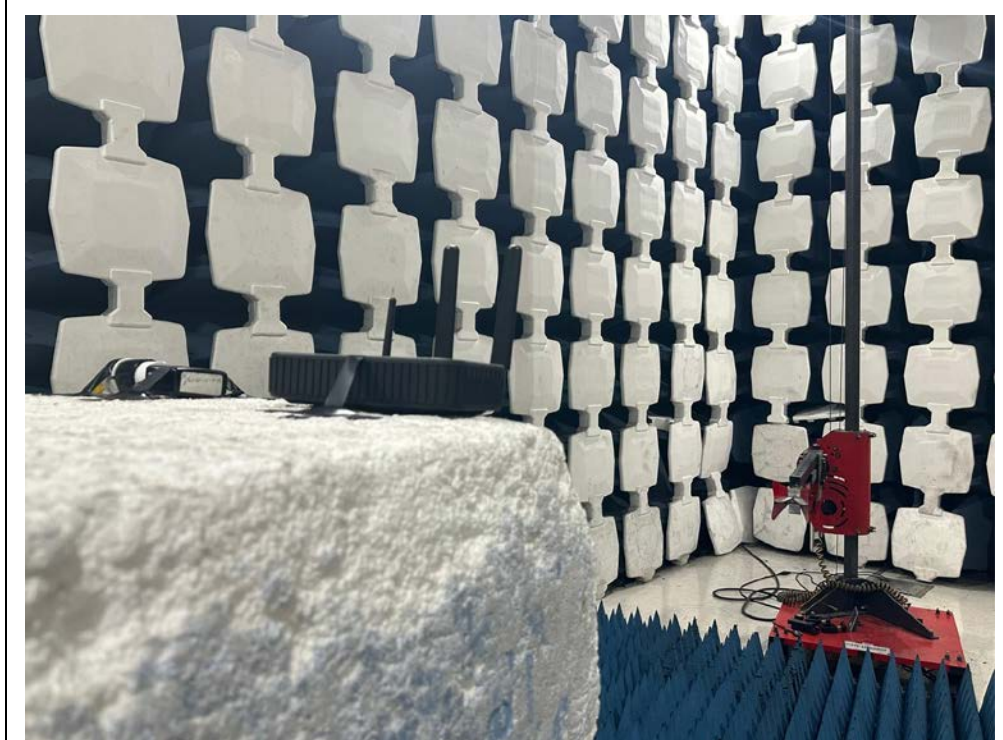
1-10GHz Rear (H4P3-TWC)
