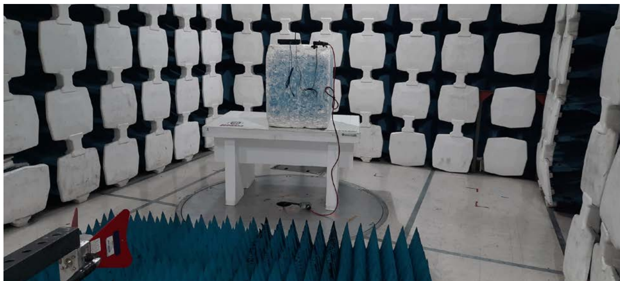
1-10GHz Front
