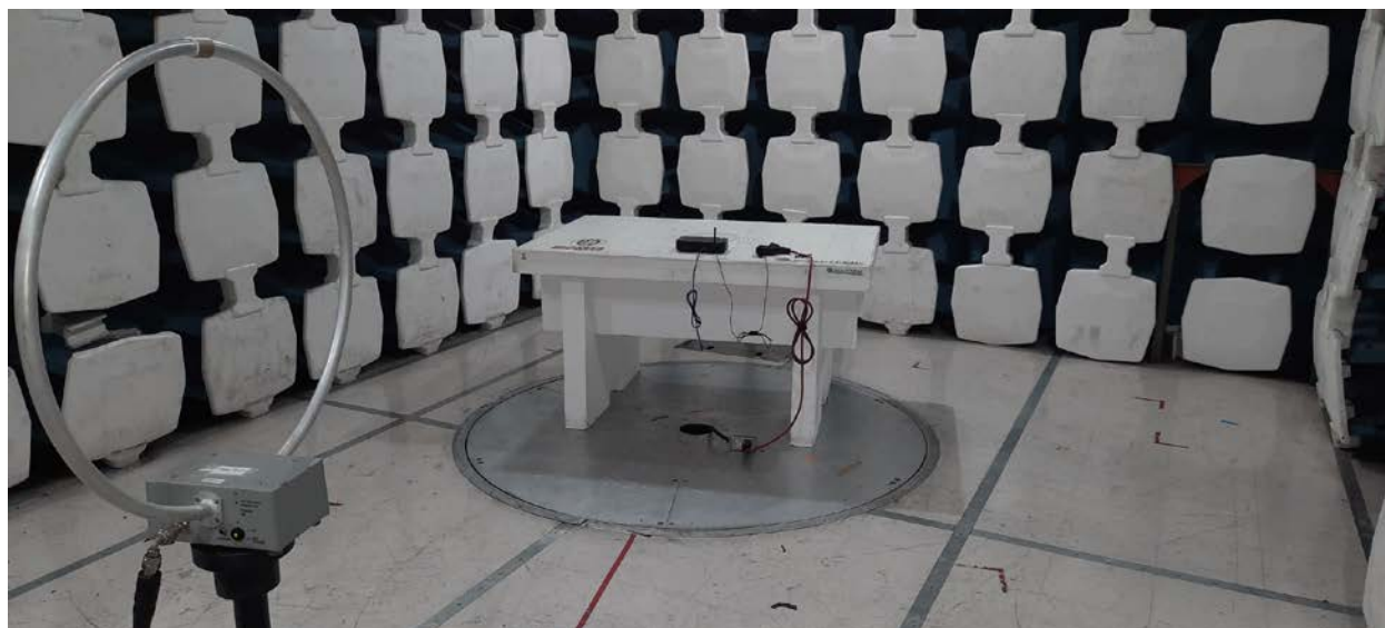
9kHz-30MHz Front
