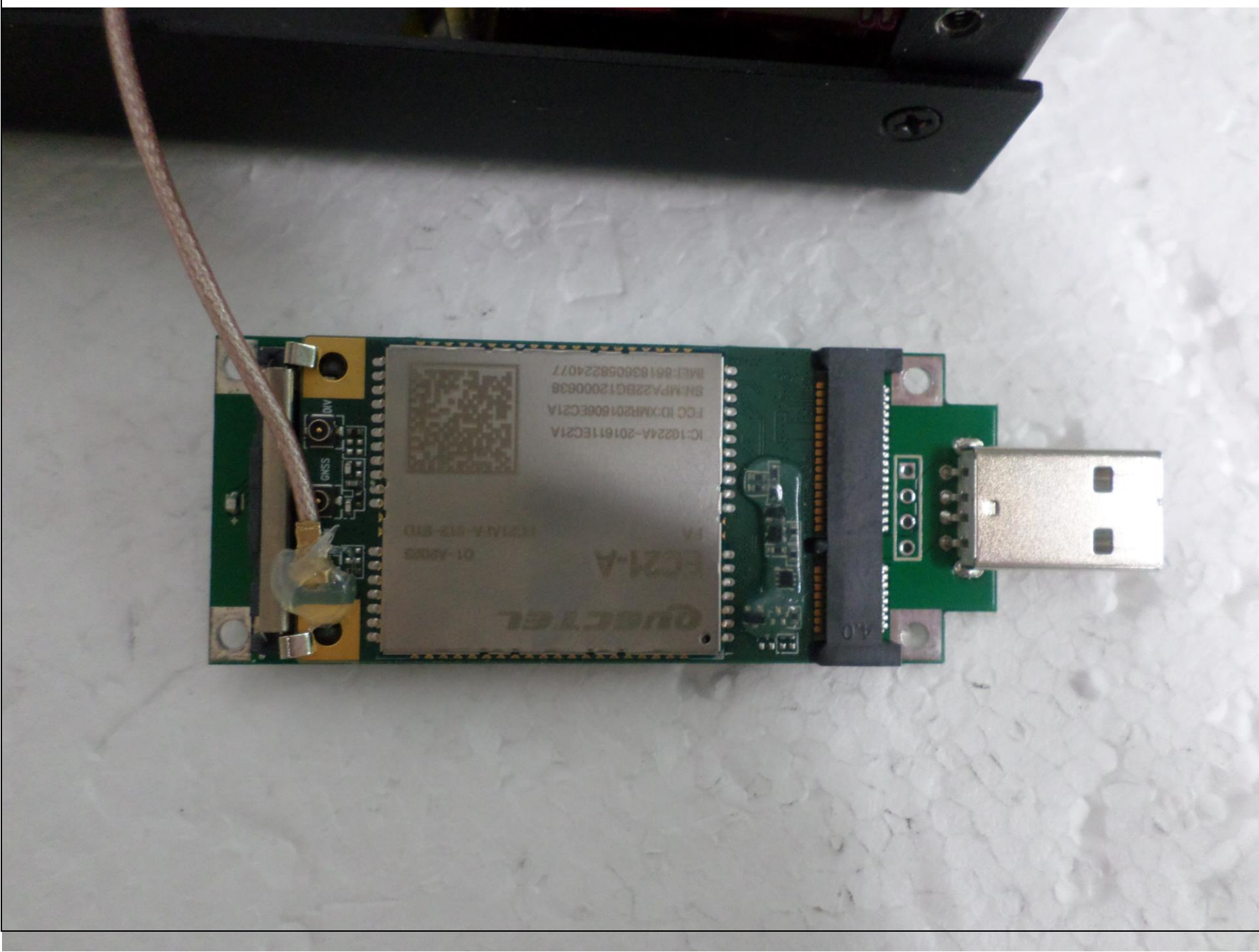
Front View of LTE Board
