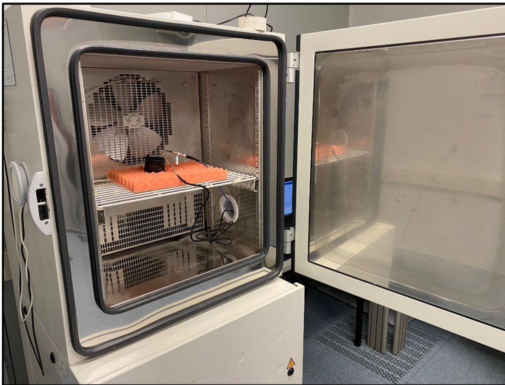
Photo 10: Conducted Test Setup-with DC Power Supply
