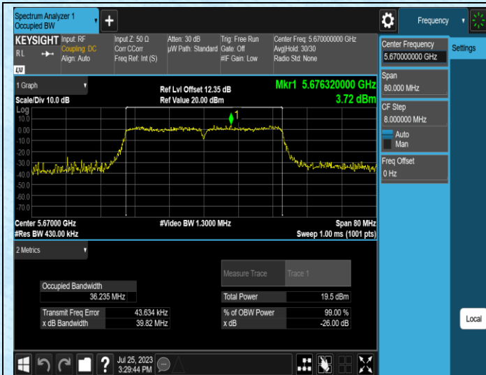
11N40SISO-Ant1-5670
