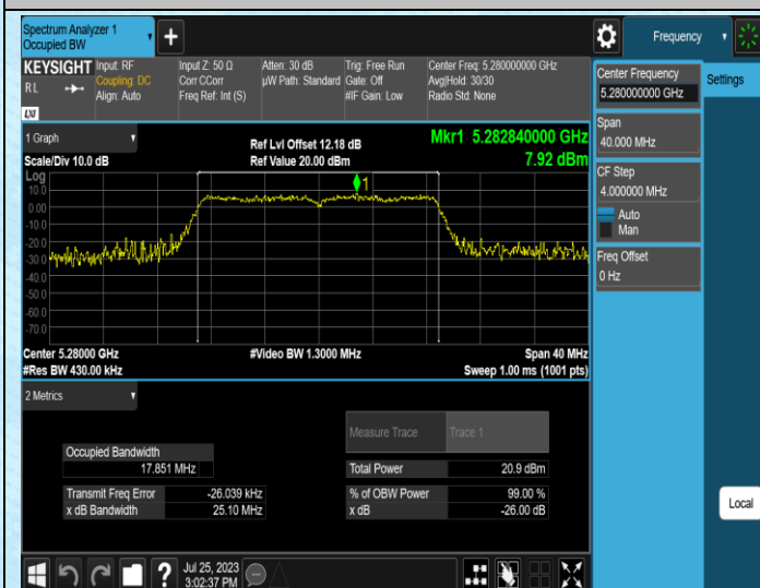
11N20SISO-Ant1-5280
