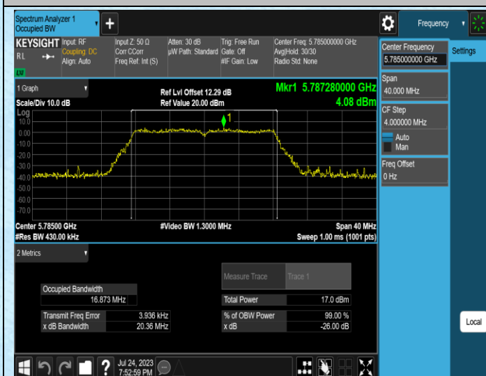
11A-Ant1-5785
