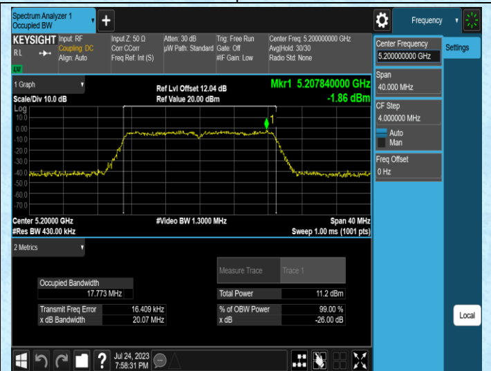
11N20SISO-Ant1-5200
