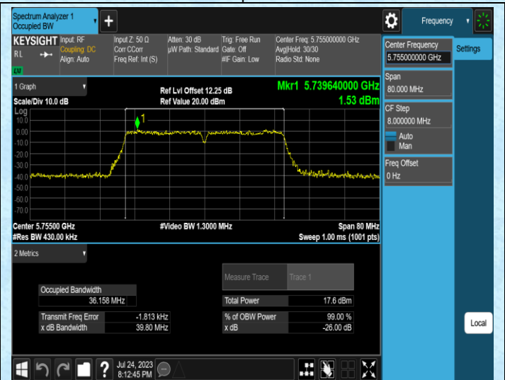
11N40SISO-Ant1-5755
