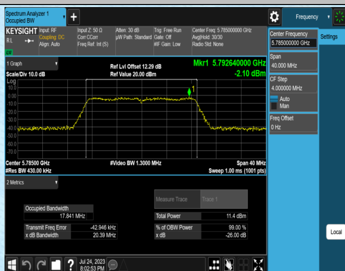
11N20SISO-Ant1-5785
