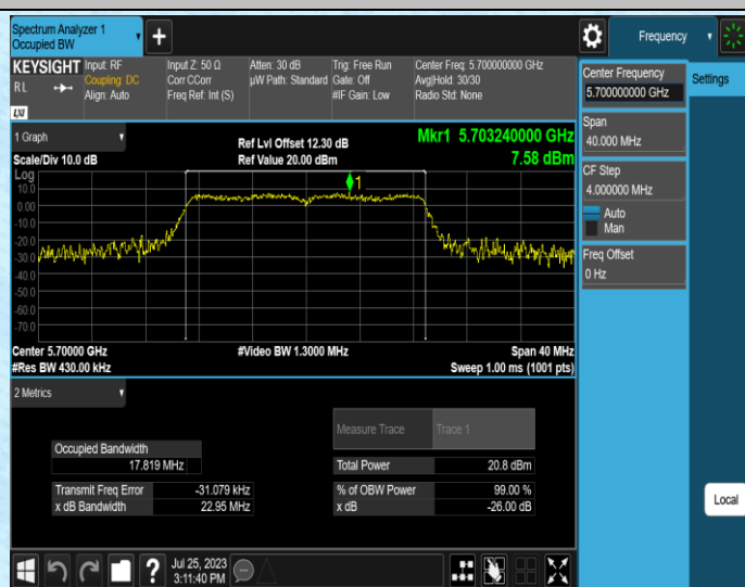
11N20SISO-Ant1-5700
