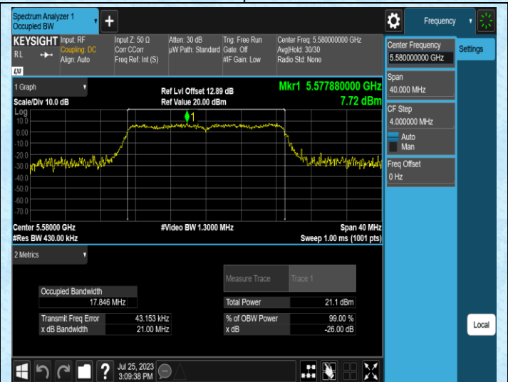
11N20SISO-Ant1-5580
