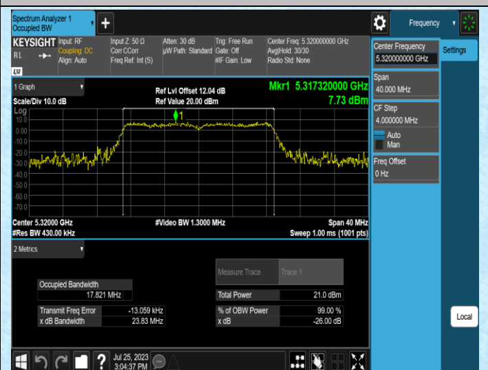
11N20SISO-Ant1-5320
