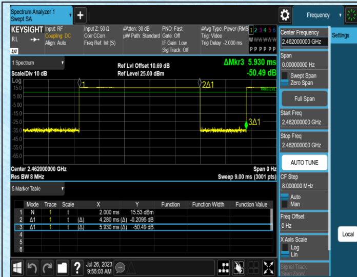
NTNV-11B-Ant1-2462
