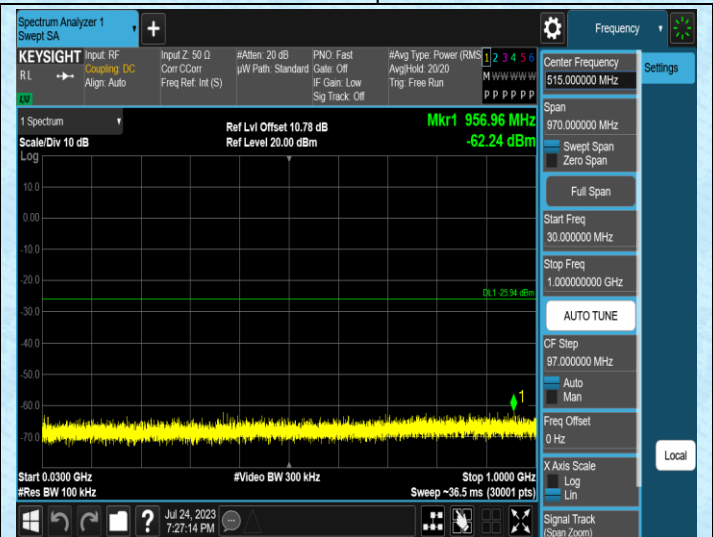
11N20SISO-Ant1-2412-30~1000
