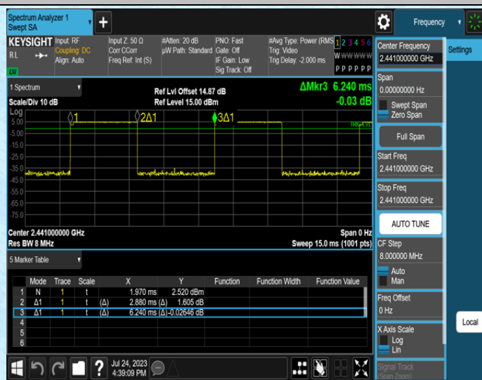
NTNV-2DH5-Ant1-2441
