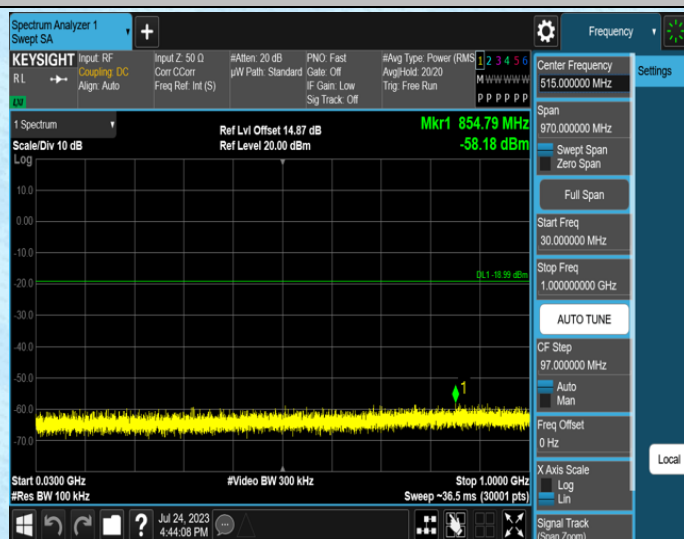
3DH5-Ant1-2441-30~1000
