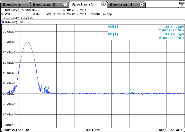
Radiated restricted band edge plot - 2 480 MHz (Average)
