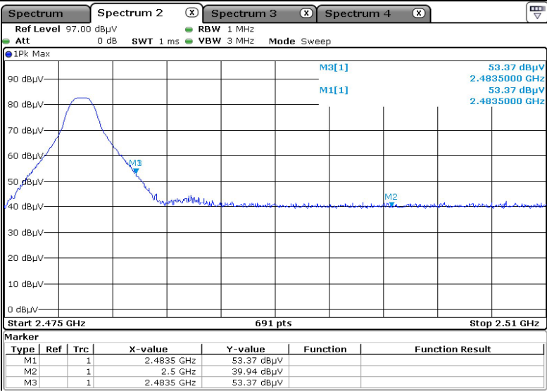
Radiated restricted band edge plot - 2 480 MHz (Peak)
