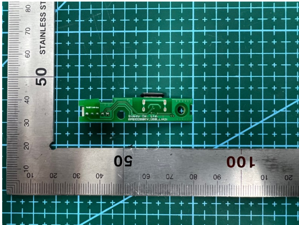
Front View of Sub Board (USB)
