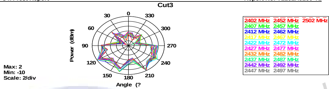
2402MHz ~2502 MHz Wi-Fi 2.4G 3D Gain
