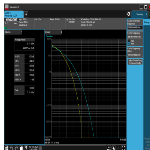
NTNV-N78-3450-3550-PC2-30-70-H-DFT-16QAM- Outer_Full-PASS
