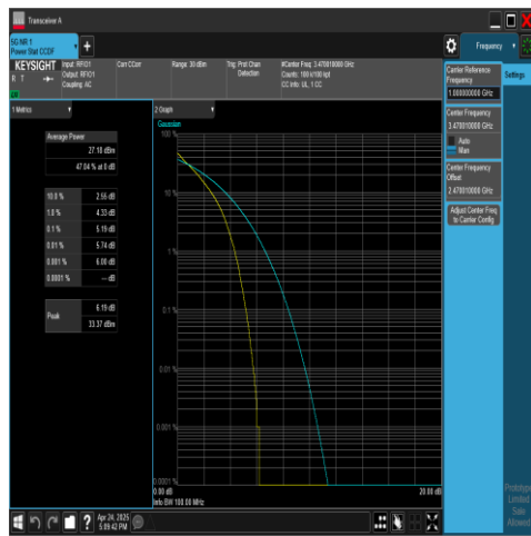
NTNV-N78-3450-3550-PC2-30-40-L-DFT-QPSK-O uter_Full-PASS
