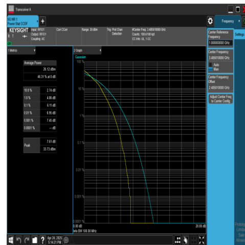
NTNV-N78-3450-3550-PC2-30-70-L-DFT-16QAM- Outer_Full-PASS
