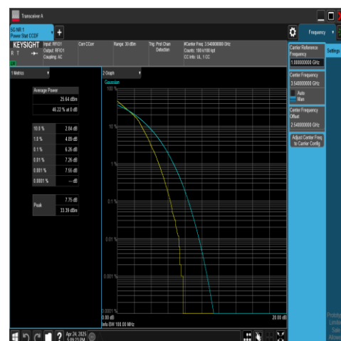
NTNV-N78-3450-3550-PC2-30-20-H-DFT-16QAM- Outer Full-PASS
