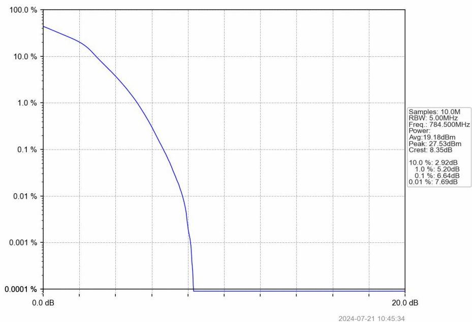
Band13_5MHz_16QAM_HCH_784.5MHz_RB_25_0_NTNV
