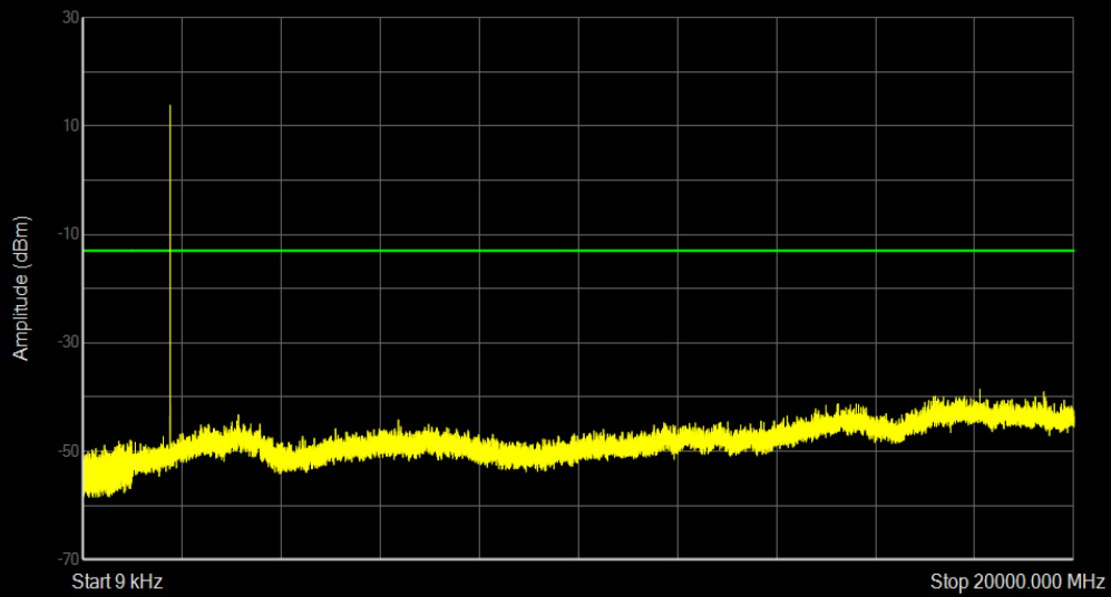
Band66 16QAM BW=1.4MHz Channel=132665 RB Size=1 Position=#0
