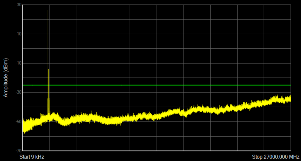
Band41 QPSK BW=20MHz Channel=40620 RB Size=1 Position=#0
