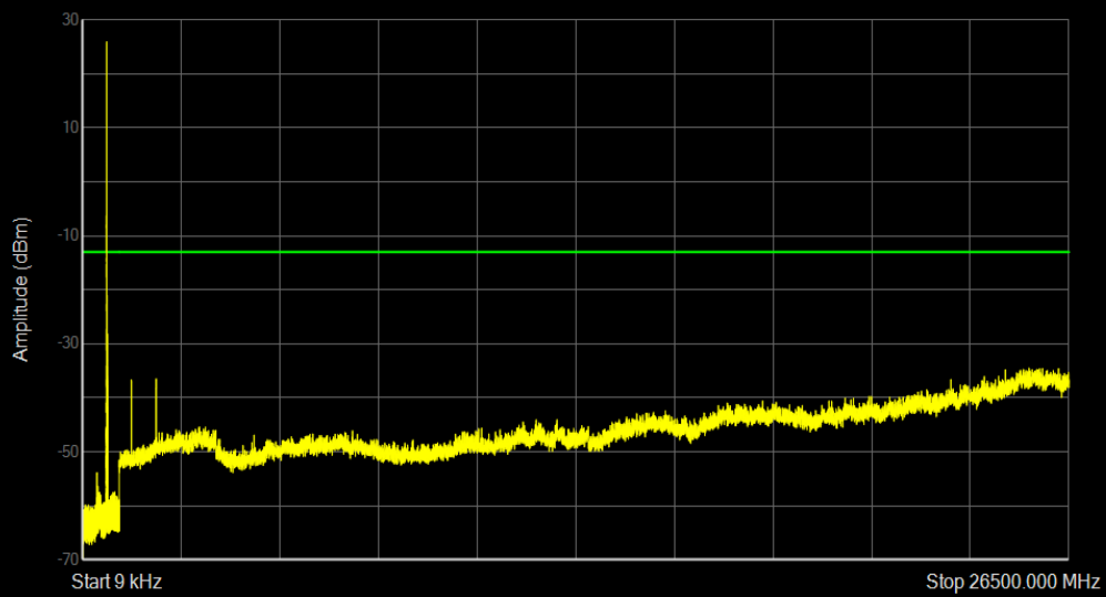
Band71 QAM16 BW=10MHz Channel=133172 RB Size=1 Position=#0
