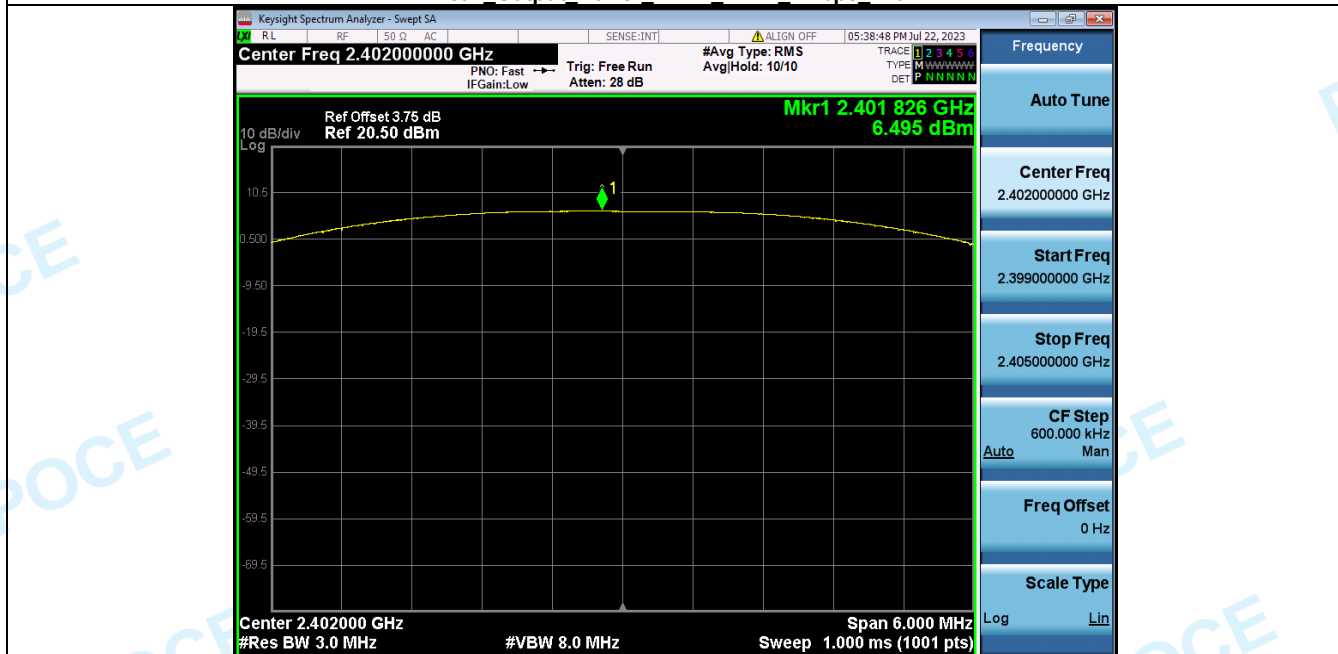
Peak Output Power NVNT ANT1 1Mbps 2402
