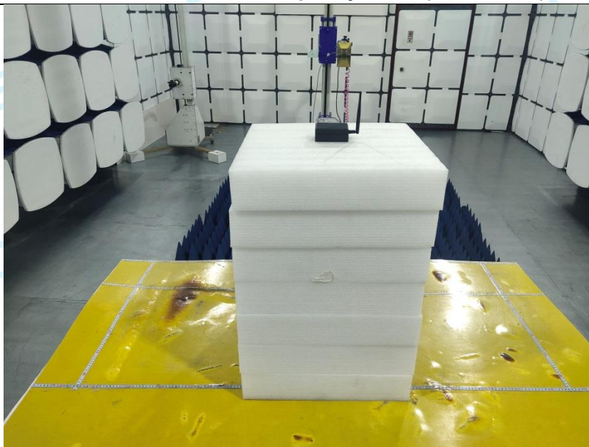
Emissions in restricted frequency bands (above 1GHz)
