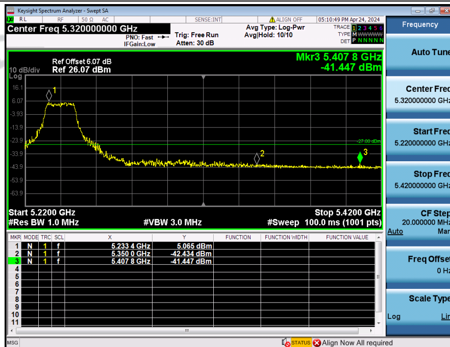
Bandedge_NVNT_ANT1_802_11a_5240
