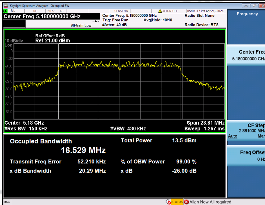
-26BW_NVNT_ANT1_802_11a_5180
