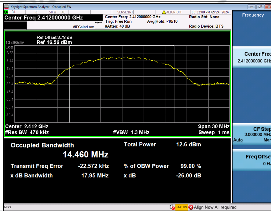
99% Occupied Bandwidth_NVNT_ANT1_802_11b_2412
