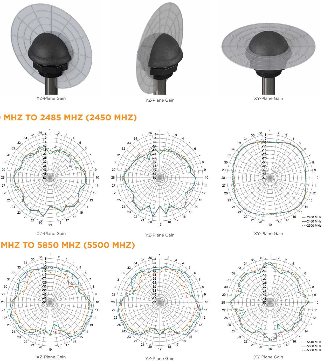
Figure 10: ANT-DB1-WRT-ccc Radiation Patterns, Free Space
