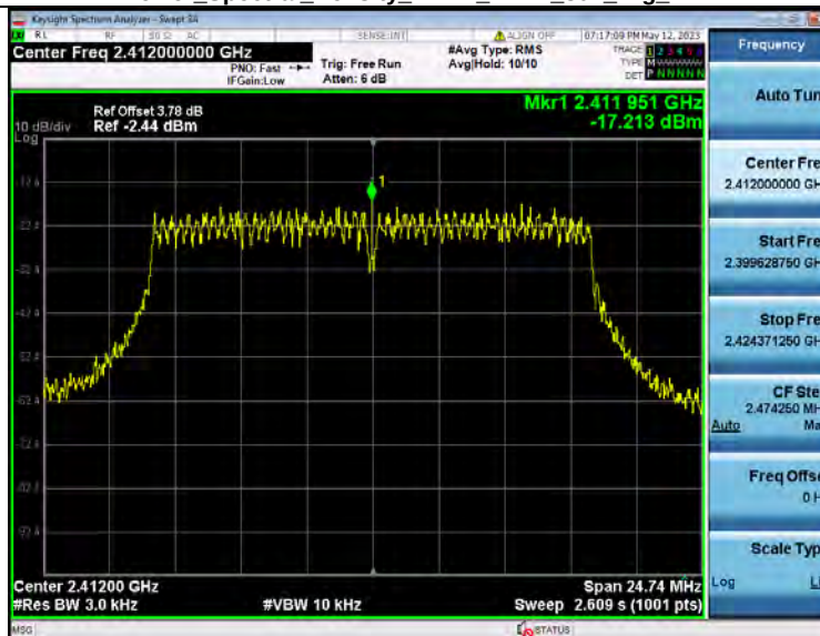
Power_Spectral_Density_NVNT_ANT1_802_11g_2412
