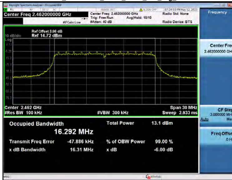
-6dB_Bandwidth_NVNT_ANT1_802_11g_2462
