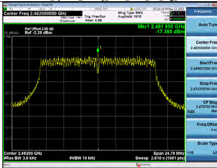
Power Spectral Density NVNT_ANT1_802_11g_2462
