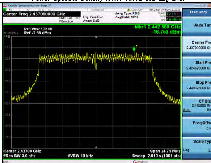
Power_Spectral_Density_NVNT_ANT1_802_11g_2437
