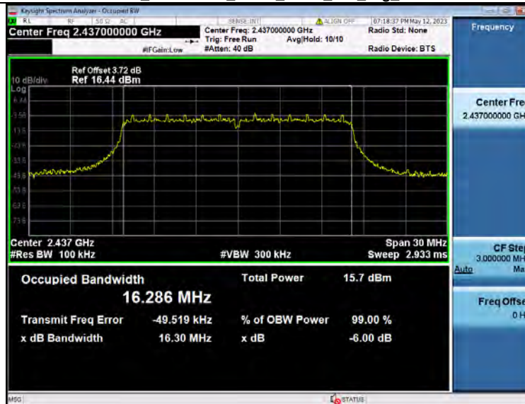
-6dB Bandwidth_NVNT ANT1_802_11g_2437
