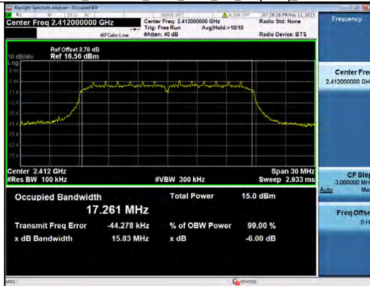
-6dB_Bandwidth_NVNT_ANT1_802_11n(HT20)_2412
