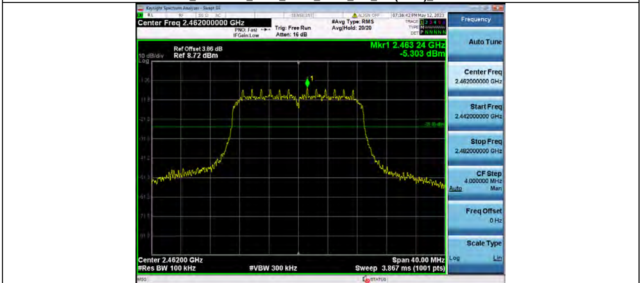
2 Bandedge_NVNT_ANT1_802_11n(HT20)_2462
