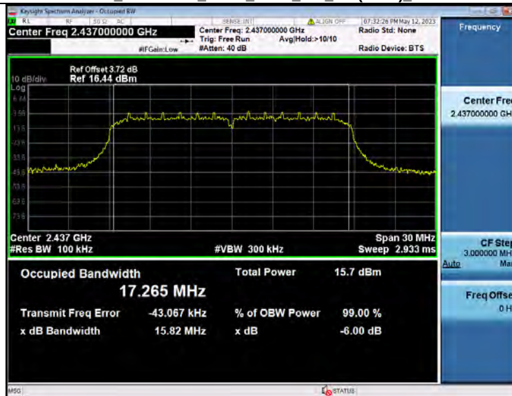
-6dB_Bandwidth_NVNT_ANT1_802_11n(HT20)_2437
