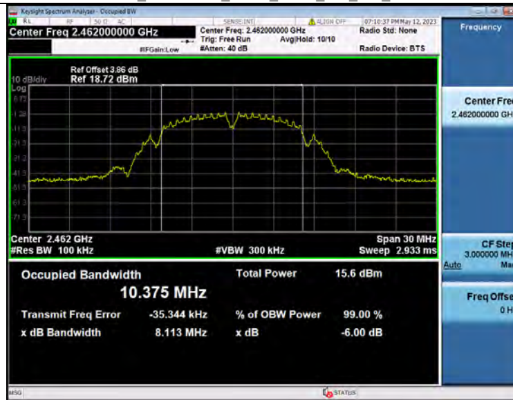
-6dB Bandwidth_NVNT_ANT1_802_11b_2462
