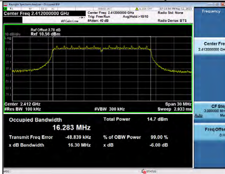
-6dB Bandwidth_NVNT_ANT1_802_11g_2412
