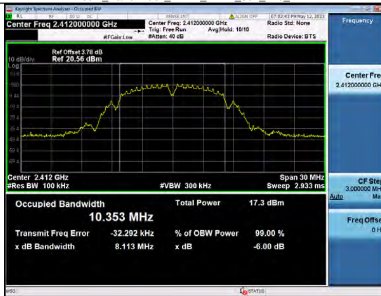
-6dB_Bandwidth_NVNT_ANT1_802_11b_2412
