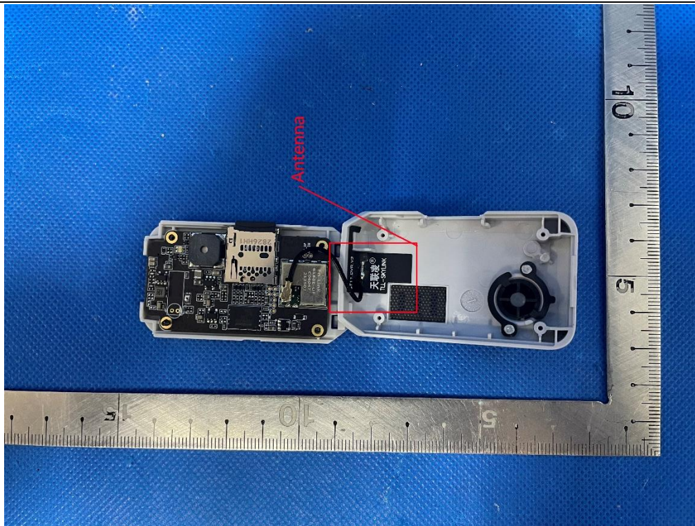
EUT Photo(6)- Antenna
