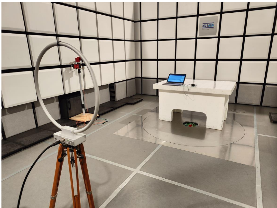
Figure 2: Spurious emission 90 kHz-30 MHz
