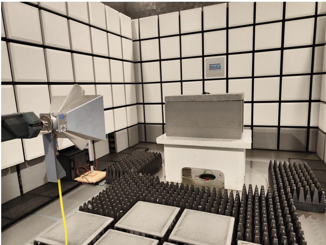
Figure 4: Spurious emission 1-18 GHz
