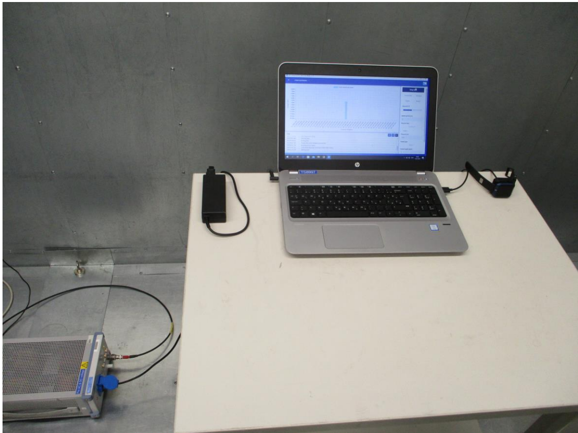
Figure 1: AC Line conducted emission
