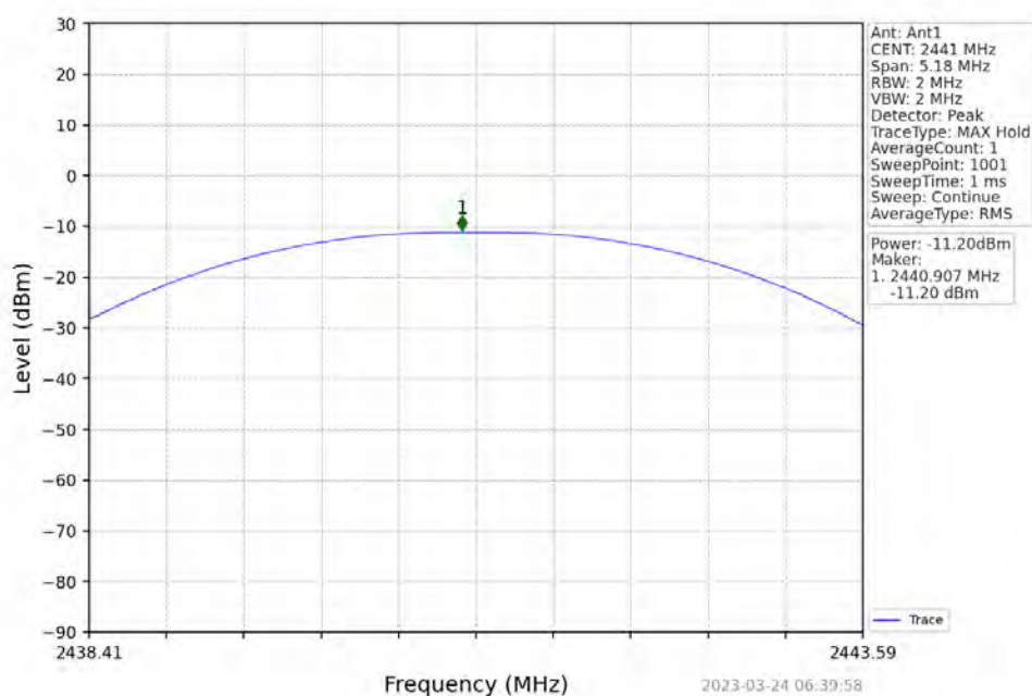
8DPSK_3DH5_MCH_2441MHz
