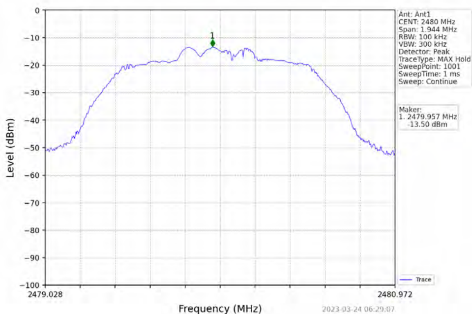
Pi/4DQPSK_2DH5_HCH_2480MHz
