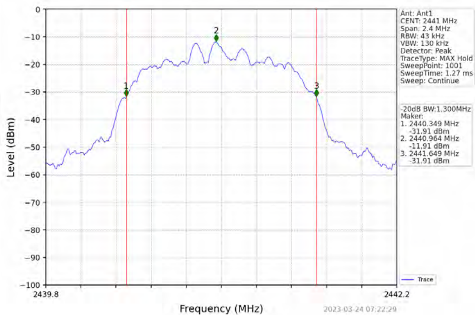
Pi/4DQPSK_2DH5_MCH_2441MHz
