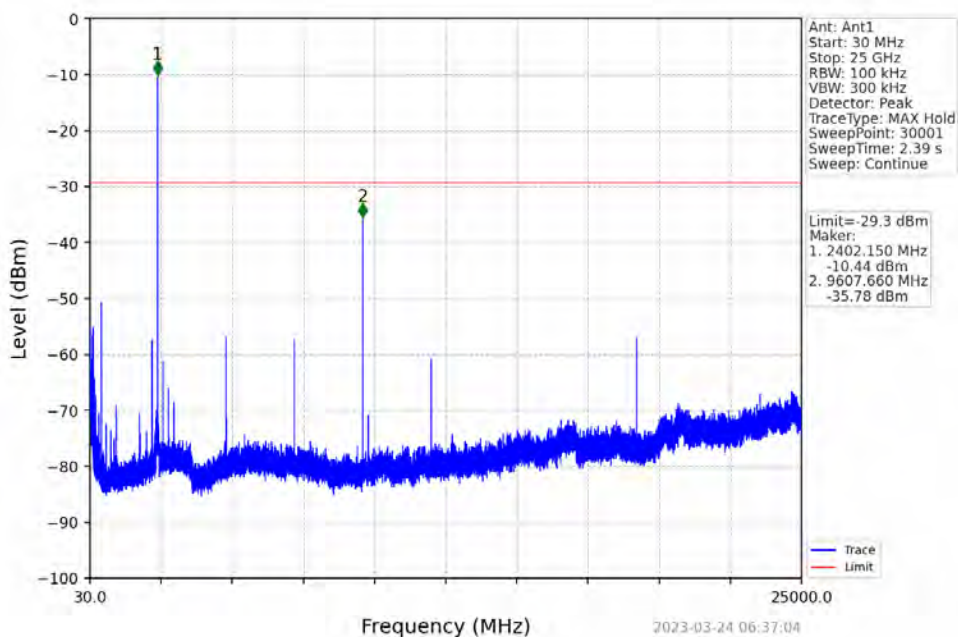
8DPSK 3DH5 LCH 2402MHz
