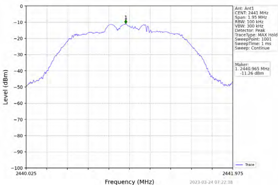
Pi/4DQPSK_2DH5_MCH_2441MHz
