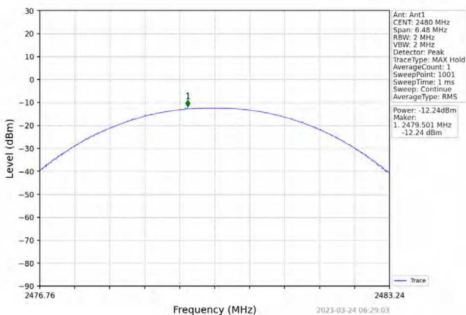
Pi/4DQPSK_2DH5_HCH_2480MHz
