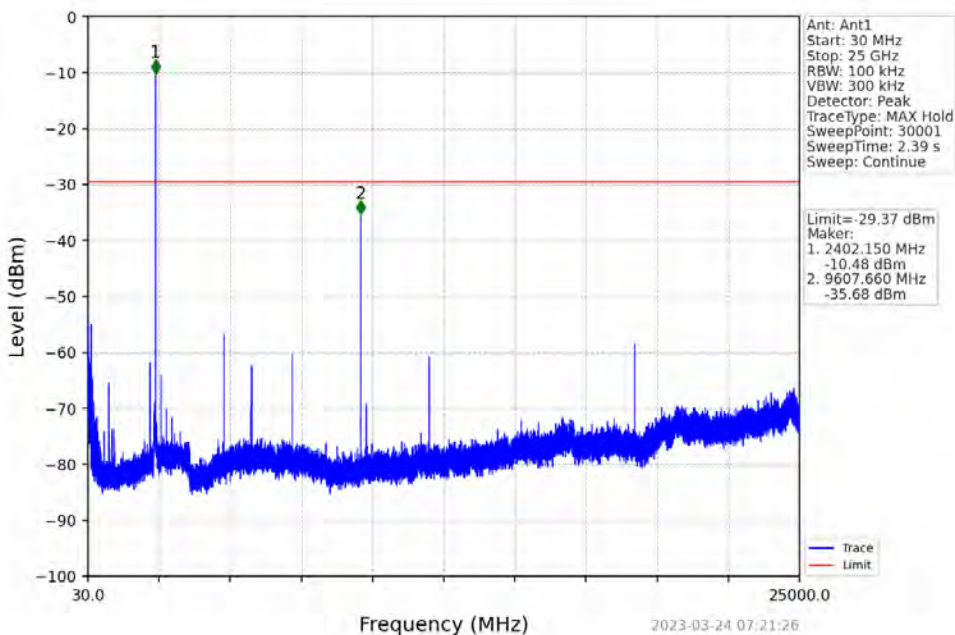
Pi/4DQPSK_2DH5_LCH_2402MHz
