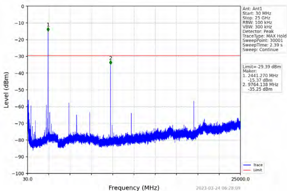
Pi/4DQPSK_2DH5_MCH_2441MHz
