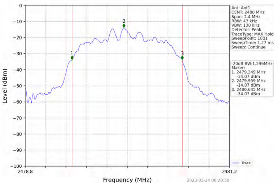
Pi/4DQPSK_2DH5_HCH_2480MHz
