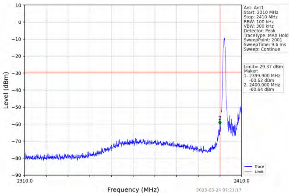
Pi/4DQPSK_2DH5_LCH_2402MHz
