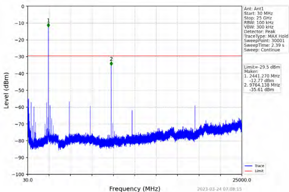
GFSK DH5 MCH 2441MHz
