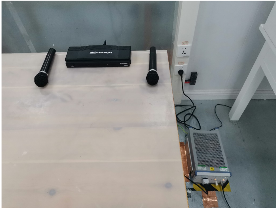
Photo of Conducted emissions Test
