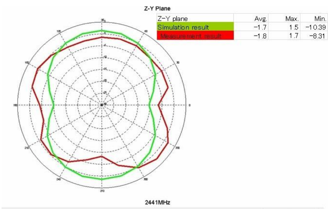
Radiation pattern @2.441GHz
