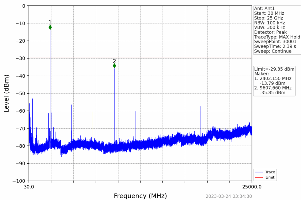
Pi/4DQPSK_2DH5_LCH_2402MHz
