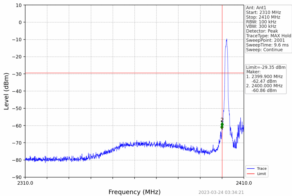
Pi/4DQPSK_2DH5_LCH_2402MHz
