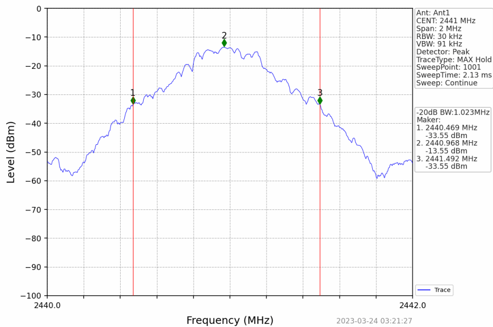
GFSK_DH5_MCH_2441MHz
