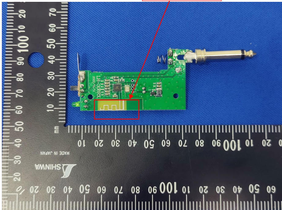
PCB Antenna
