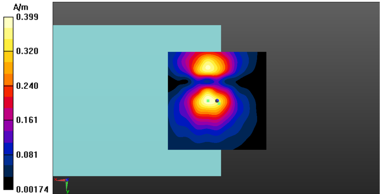
Fig A.13 T-Coil WLAN 5.2GHz-Y
