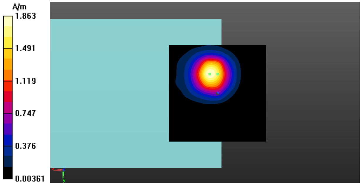
Fig A.19 T-Coil LTE-Band 66-Z
