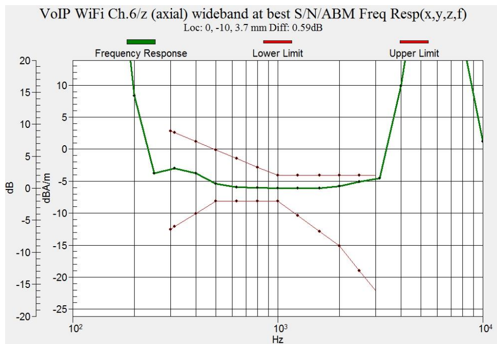
Figure B.20 Frequency Response of WLAN 2.4GHz (Google Meet)
