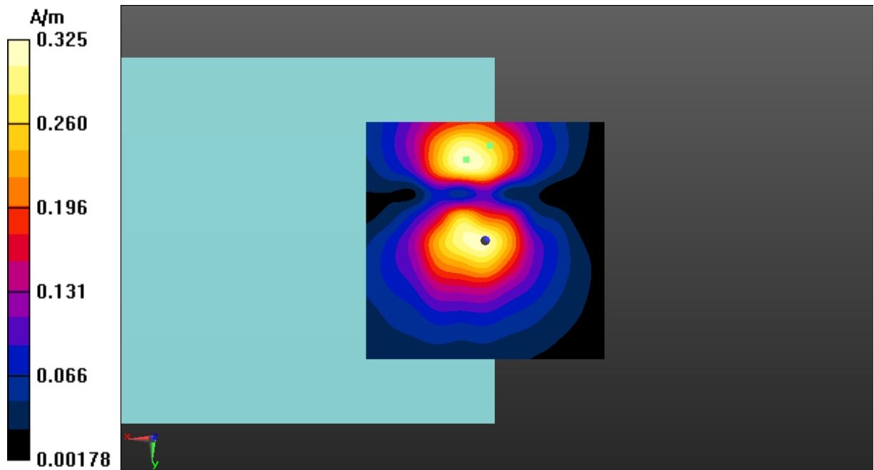
Fig A.10 T-Coil LTE-Band 66-Y
