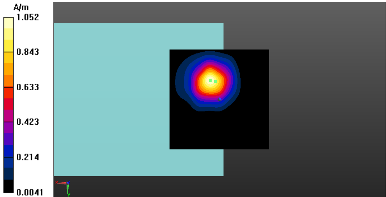
Fig A.15 T-Coil WLAN 5.5GHz-Z
