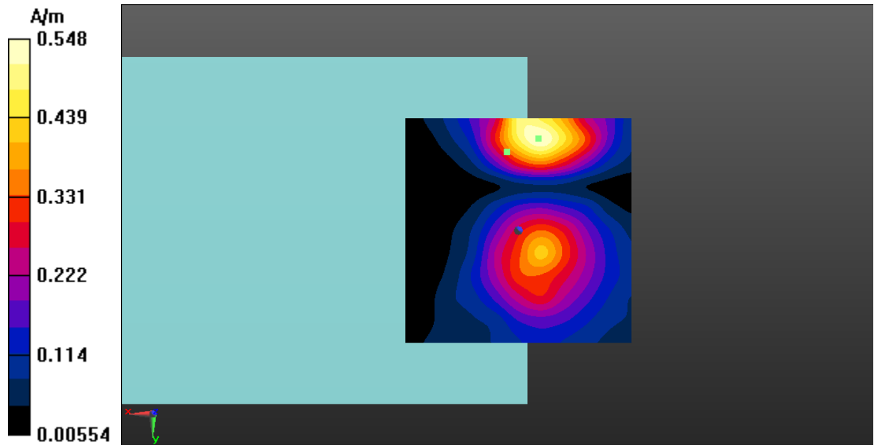
Fig A.19 T-Coil LTE-Band 66-Y
