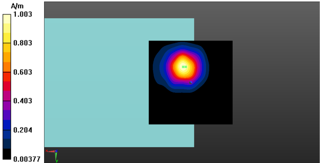
Fig A.13 T-Coil WLAN 5.2GHz-Z
