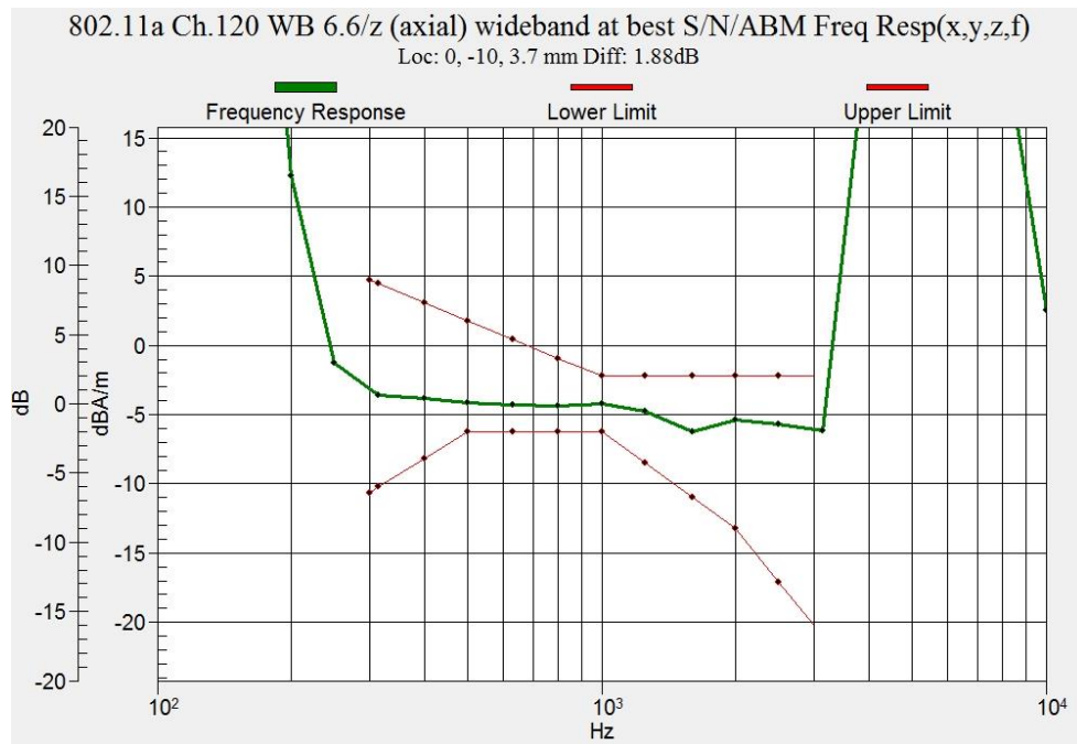
Figure B.15 Frequency Response of WLAN 5.5GHz
