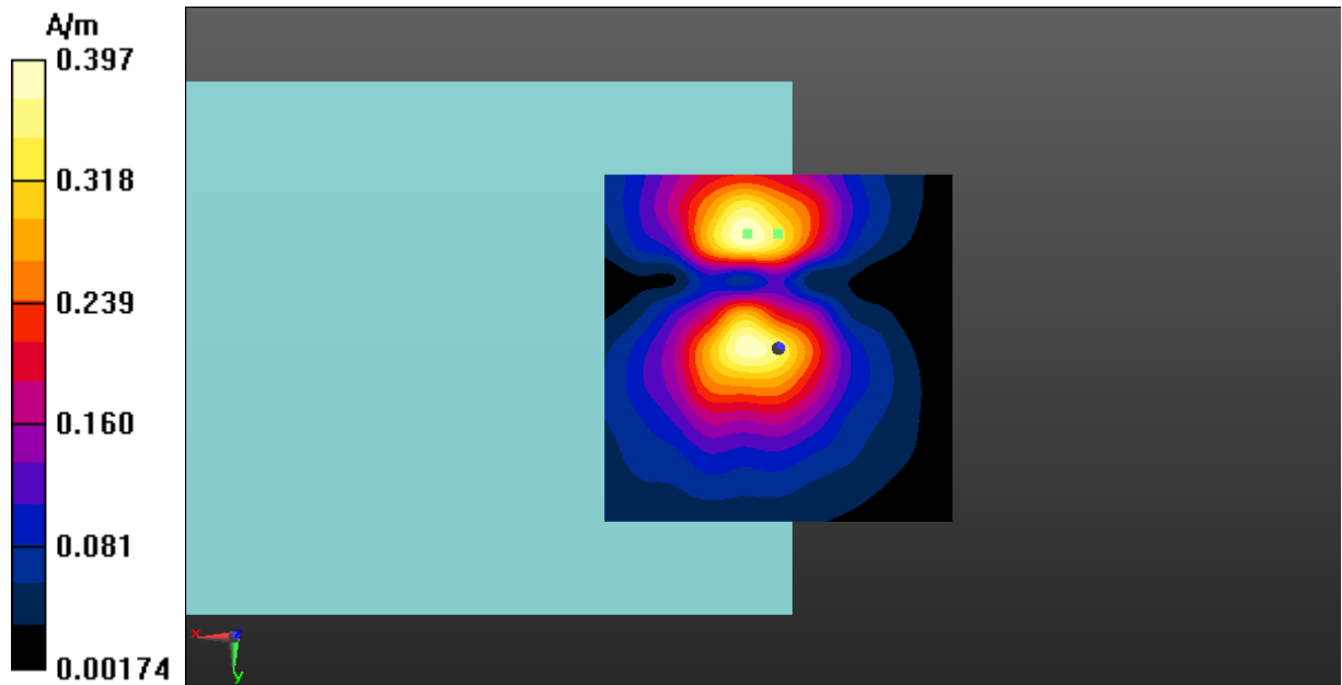
Fig A.16 T-Coil WLAN 5.8GHz-Y
