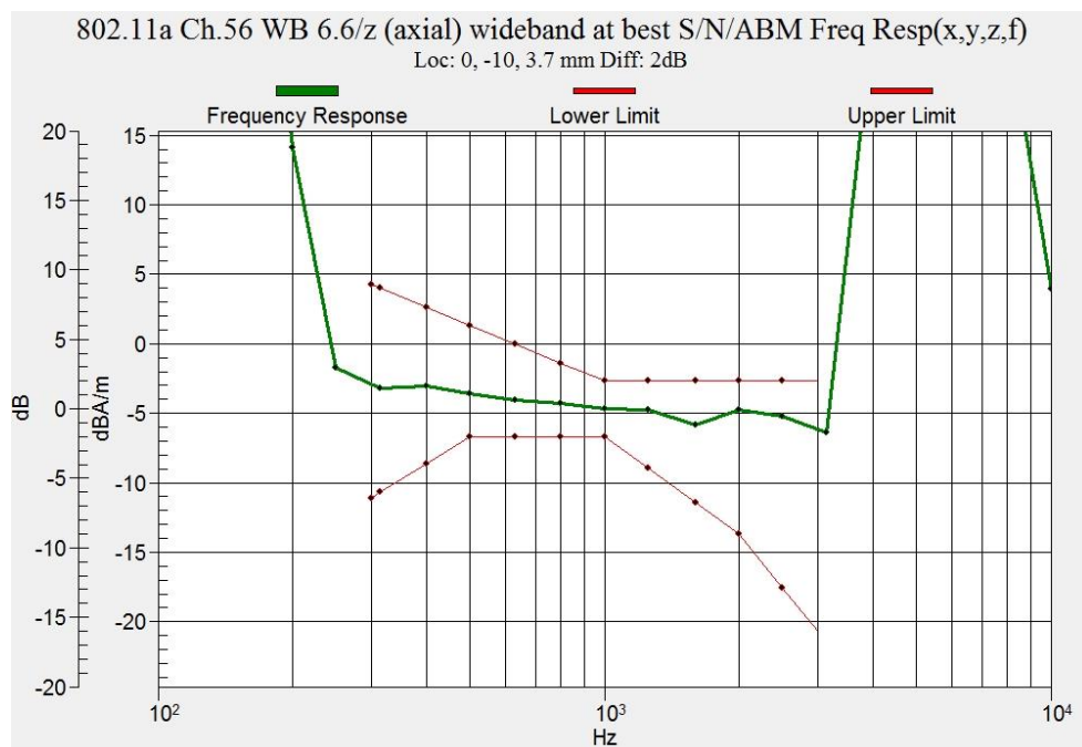
Figure B.14 Frequency Response of WLAN 5.3GHz
