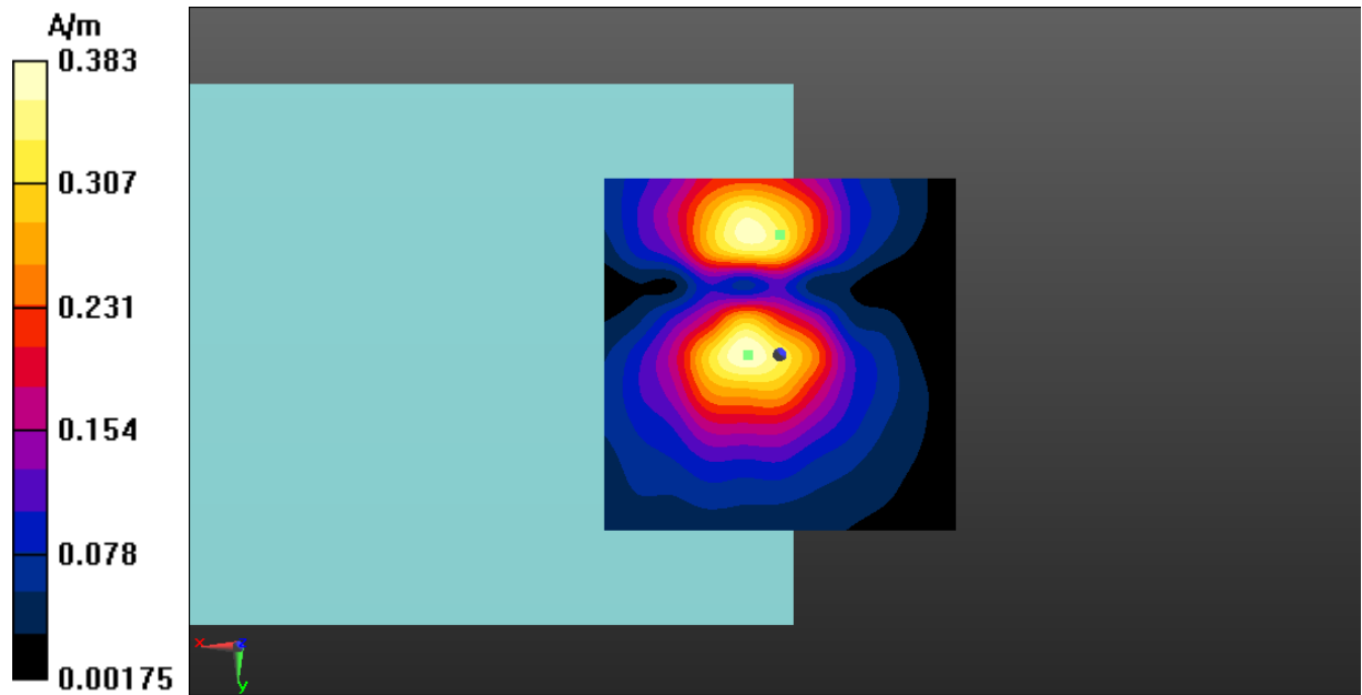
Fig A.15 T-Coil WLAN 5.5GHz-Y
