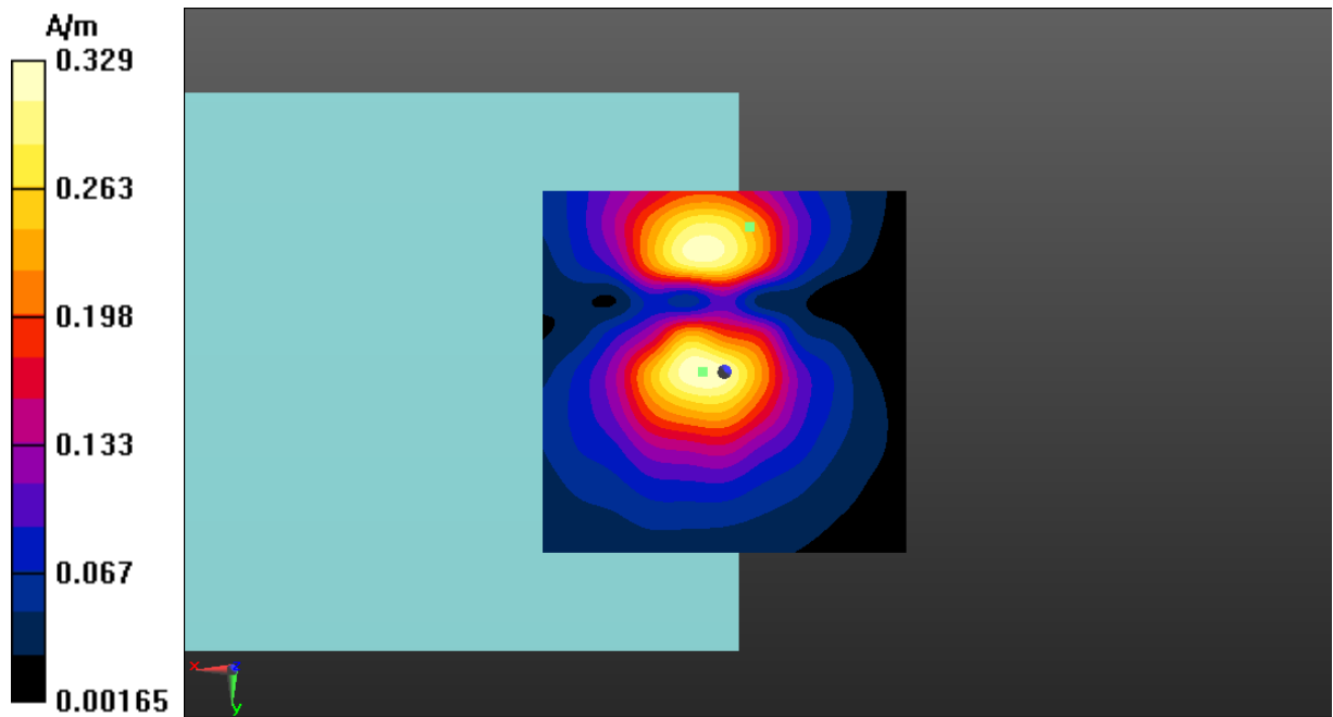
Fig A.11 T-Coil LTE-Band 71-Y
