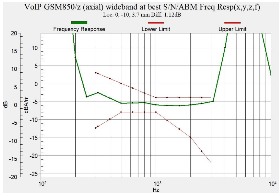
Figure B.17 Frequency Response of GSM 850 (Google Meet)
