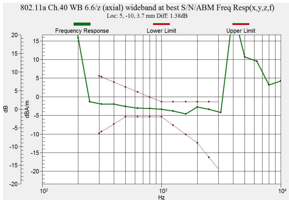
Figure B.13 Frequency Response of WLAN 5.2GHz
