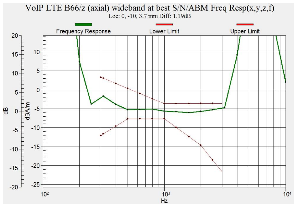
Figure B.19 Frequency Response of LTE Band 66 (Google Meet)
