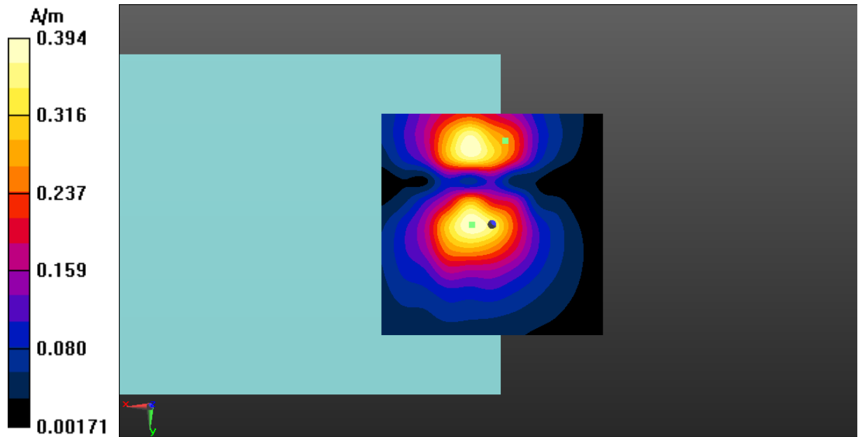
Fig A.14 T-Coil WLAN 5.3GHz-Y
