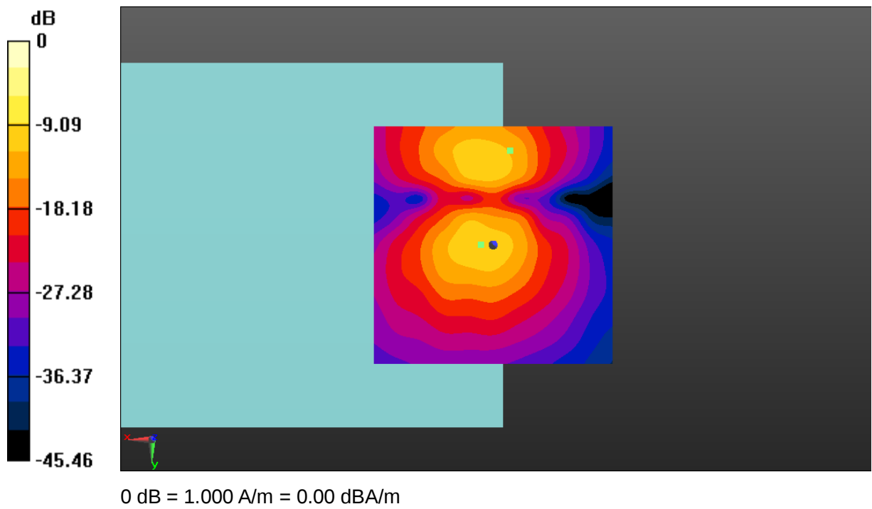
Fig A.9 T-Coil LTE-Band 12-Y
