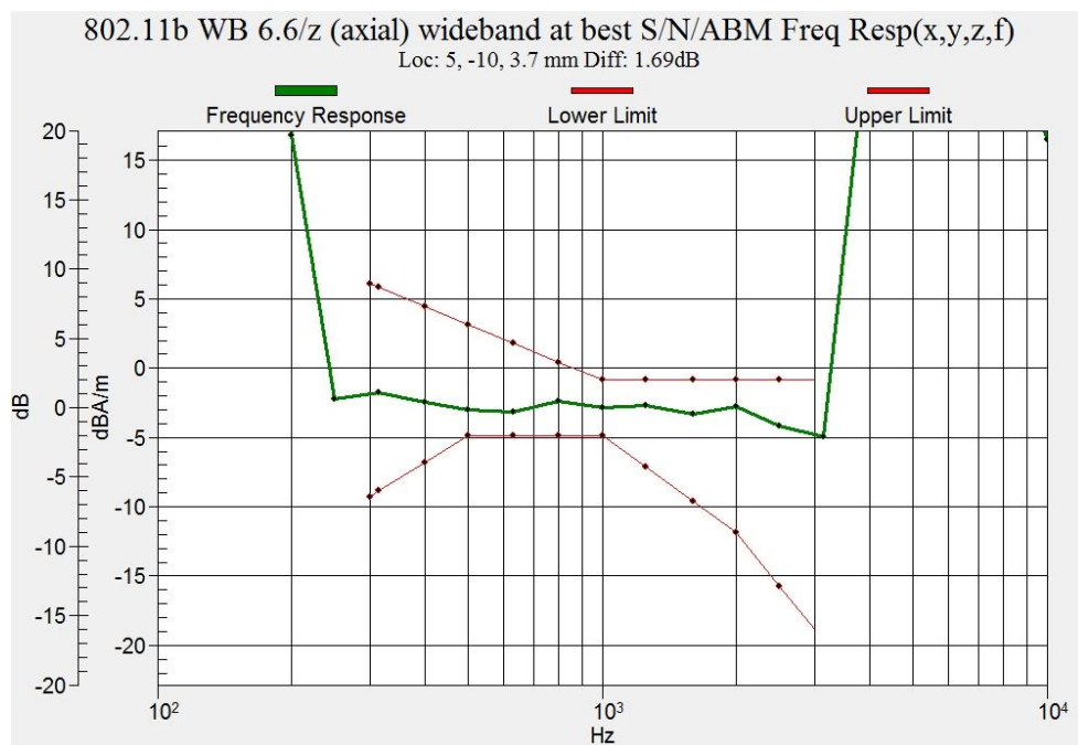
Figure B.12 Frequency Response of WLAN 2.4GHz
