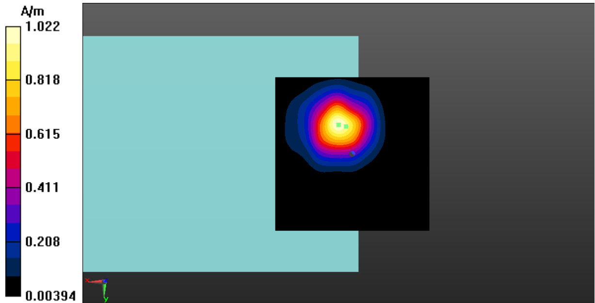
Fig A.14 T-Coil WLAN 5.3GHz-Z
