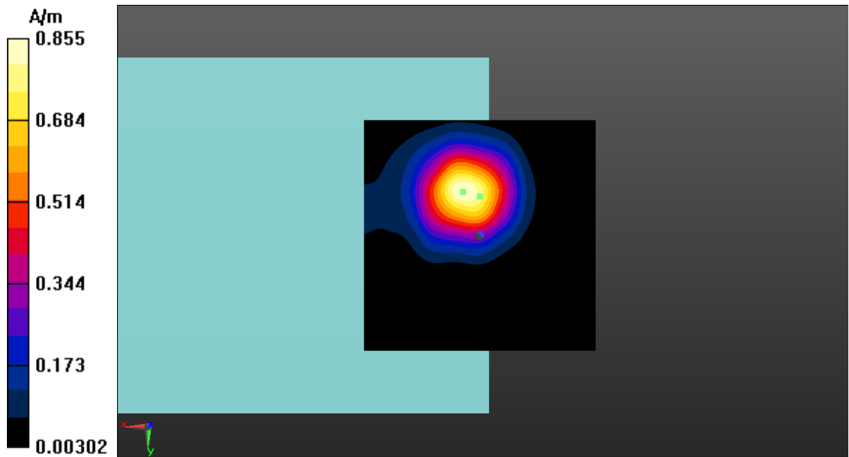
Fig A.10 T-Coil LTE-Band 66-Z
