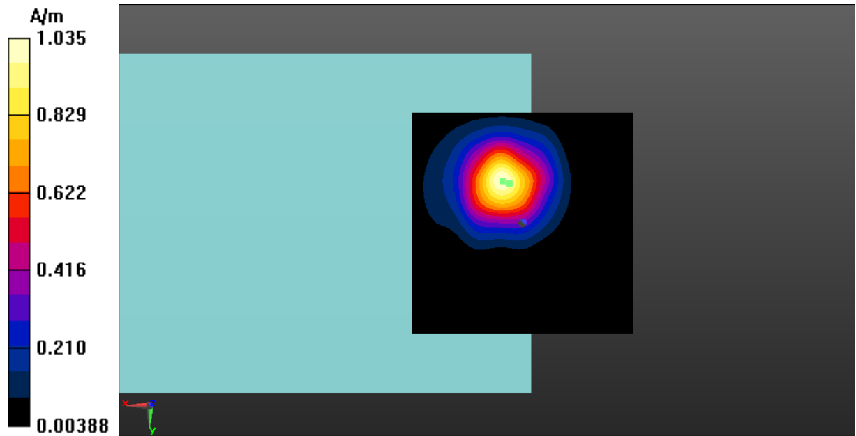
Fig A.16 T-Coil WLAN 5.8GHz-Z
