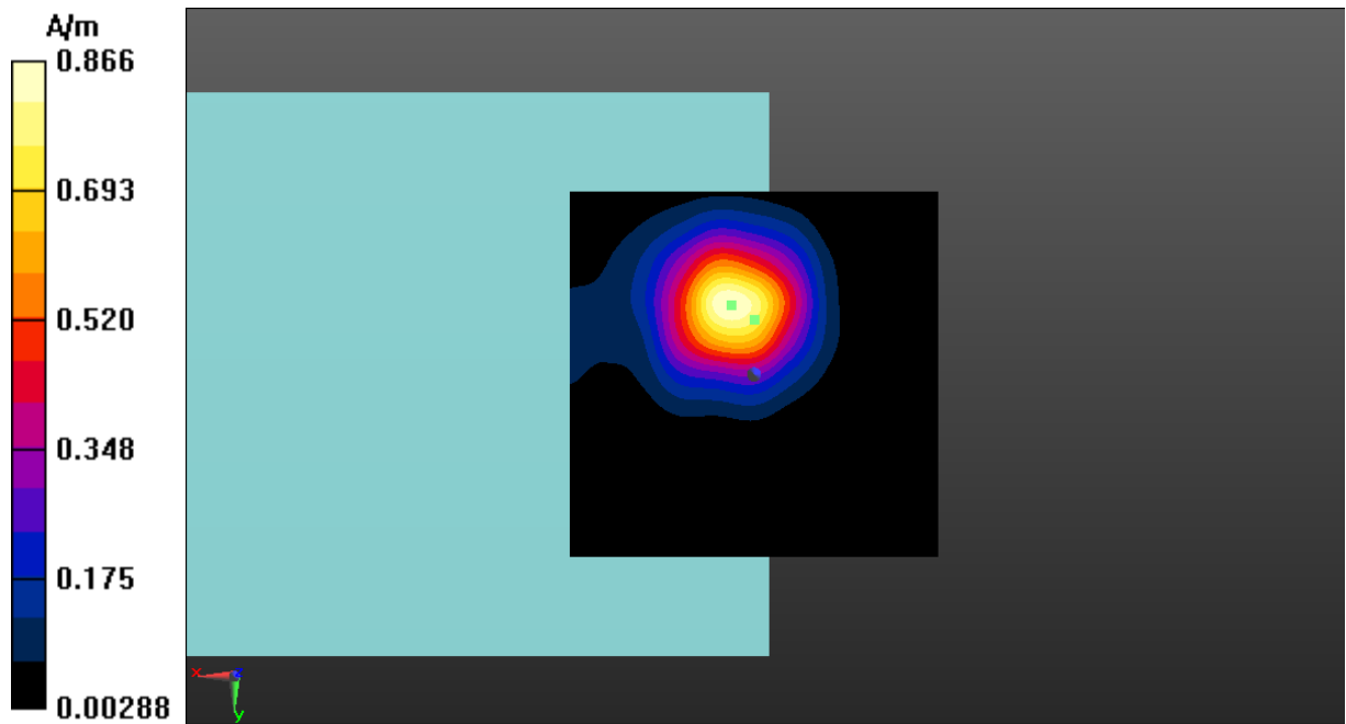
Fig A.11 T-Coil LTE-Band 71-Z
