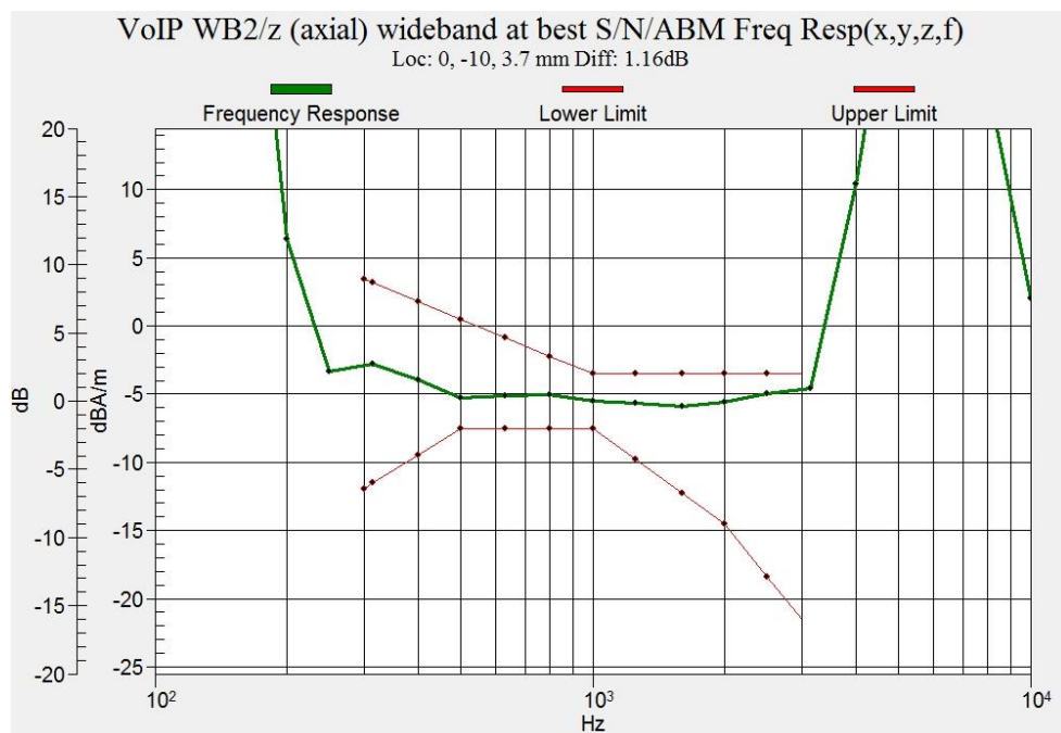
Figure B.18 Frequency Response of WCDMA Band 4 (Google Meet)
