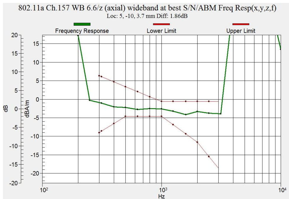
Figure B.16 Frequency Response of WLAN 5.8GHz
