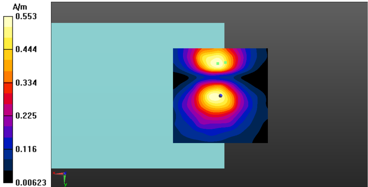
Fig A.20 T-Coil WLAN 2.4GHz-Y
