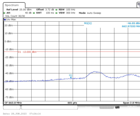
Band71-5MHz-16QAM-133147-1RB#24
