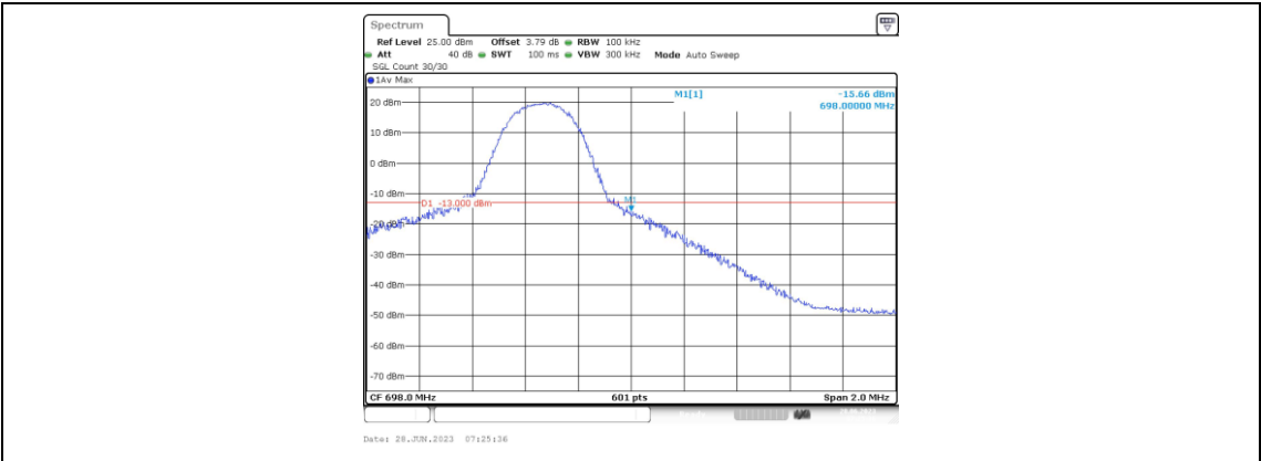
Band71-5MHz-16QAM-133447-1RB#24
