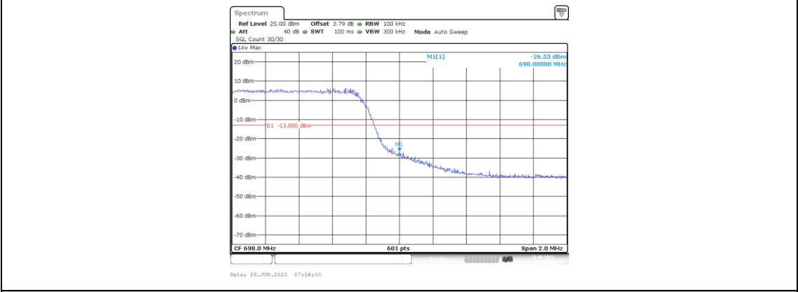
Band71-5MHz-16QAM-133447-25RB#0
