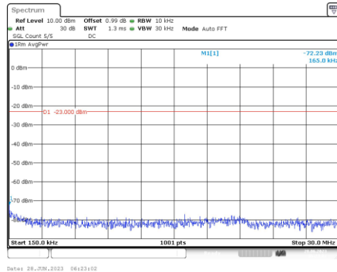
Band66-15MHz-16QAM-132597-1RB#0-Range2:0.15~30MHz
