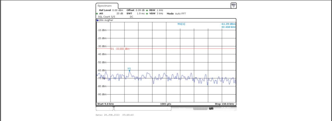
Band66-10MHz-QPSK-132622-1RB#0-Range1:0.009~0.15MHz
