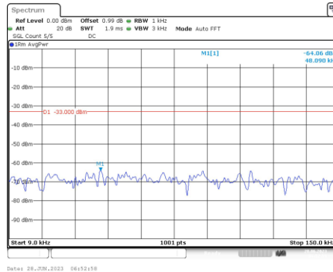
Band66-20MHz-16QAM-132072-1RB#0-Range1:0.009~0.15MHz
