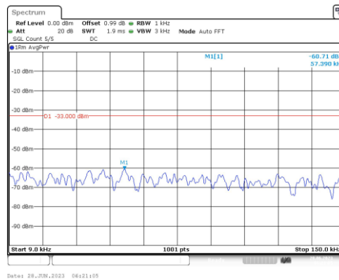
Band66-15MHz-16QAM-132322-1RB#0-Range1:0.009~0.15MHz
