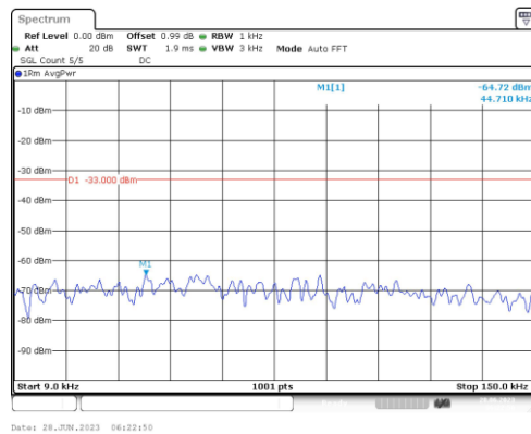
Band66-15MHz-16QAM-132597-1RB#0-Range1:0.009~0.15MHz
