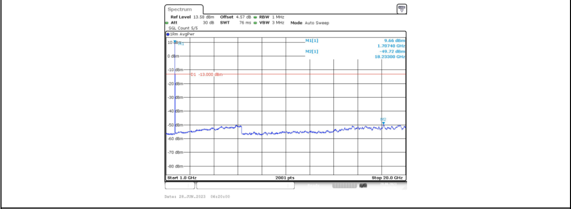
Band66-15MHz-16QAM-132047-1RB#0-Range4:1000~20000MHz
