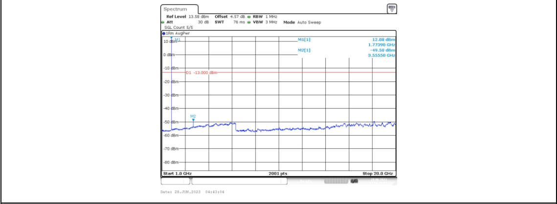
Band66-3MHz-16QAM-132657-1RB#0-Range4:1000~20000MHz
