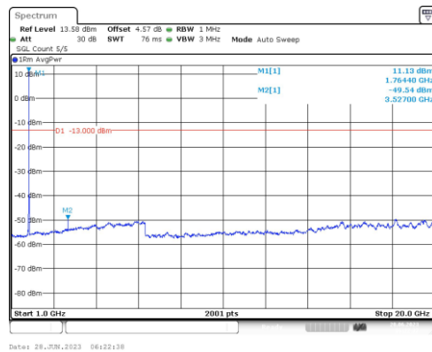
Band66-15MHz-QPSK-132597-1RB#0-Range4:1000~20000MHz
