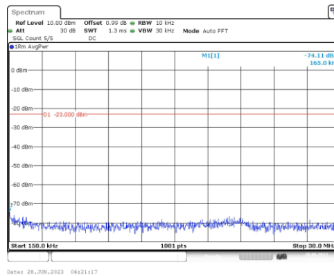
Band66-15MHz-16QAM-132322-1RB#0-Range2:0.15~30MHz
