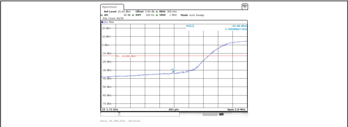
Band66-15MHz-QPSK-132047-75RB#0
