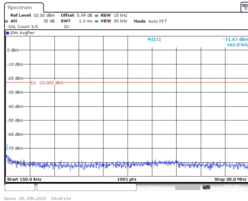
Band66-3MHz-QPSK-132322-1RB#0-Range2:0.15~30MHz
