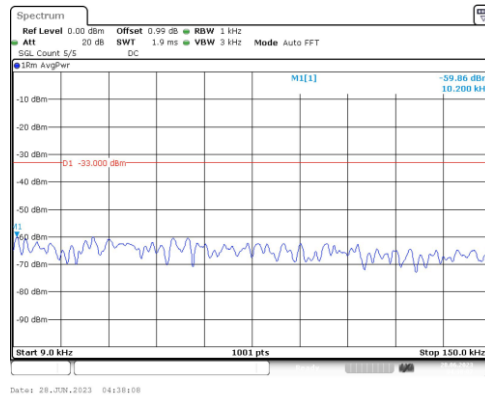
Band66-3MHz-QPSK-131987-1RB#0-Range1:0.009~0.15MHz
