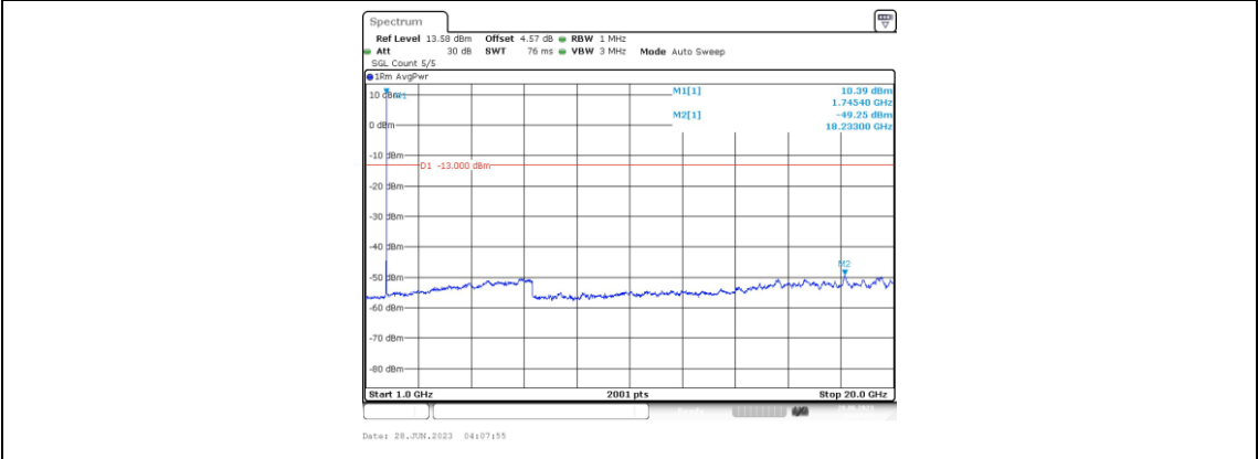
Band66-1.4MHz-QPSK-132322-1RB#0-Range4:1000~20000MHz
