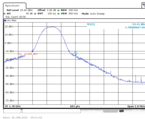
Band66-5MHz-16QAM-132647-1RB#24
