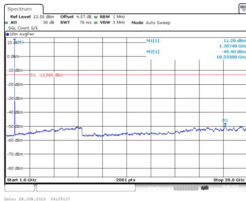
Band66-3MHz-16QAM-131987-1RB#0-Range4:1000~20000MHz
