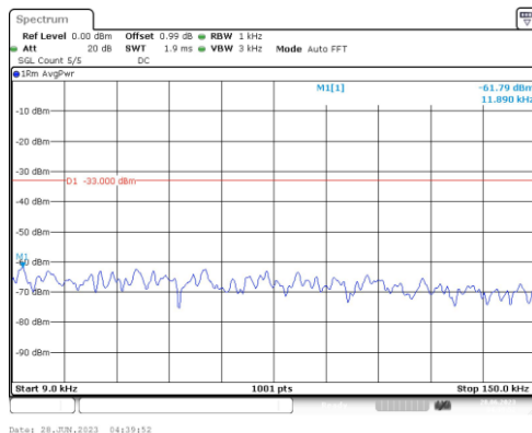
Band66-3MHz-QPSK-132322-1RB#0-Range1:0.009~0.15MHz
