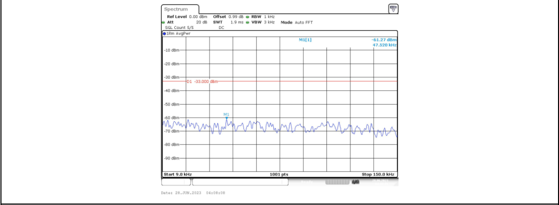
Band66-1.4MHz-16QAM-132322-1RB#0-Range1:0.009~0.15MHz
