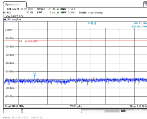
Band66-3MHz-QPSK-131987-1RB#0-Range3:30~1000MHz
