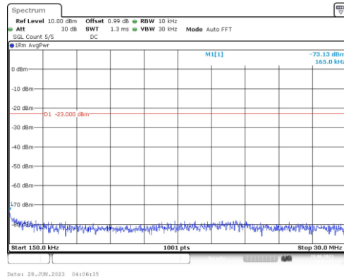
Band66-1.4MHz-16QAM-131979-1RB#0-Range2:0.15~30MHz
