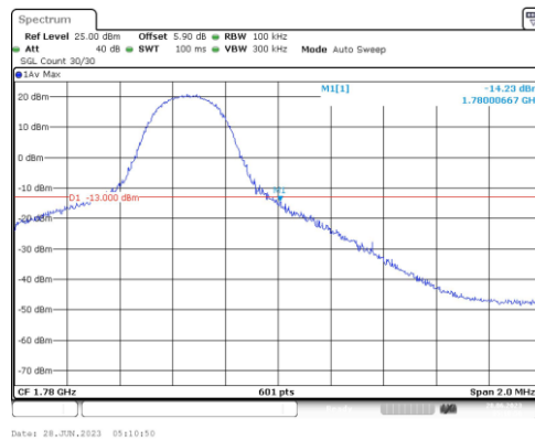
Band66-5MHz-QPSK-132647-1RB#24
