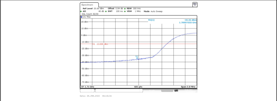
Band66-15MHz-16QAM-132047-75RB#0
