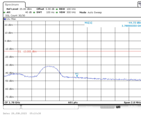
Band66-5MHz-16QAM-132647-1RB#0
