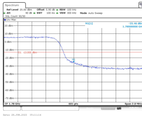
Band66-5MHz-16QAM-132647-1RB#24
