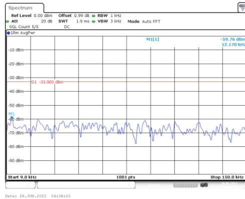
Band66-1.4MHz-16QAM-131979-1RB#0-Range1:0.009~0.15MHz
