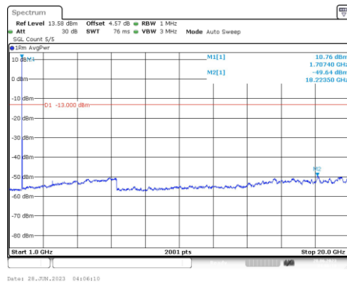
Band66-1.4MHz-QPSK-131979-1RB#0-Range4:1000~20000MHz
