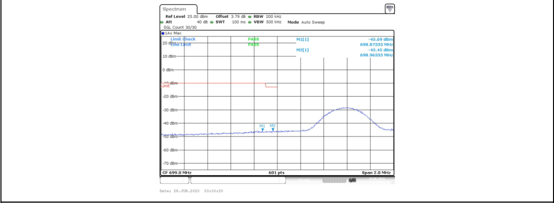
Band12-10MHz-16QAM-23060-1RB#49
