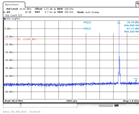
Band5-3MHz-16QAM-20635-1RB#0-Range3:30~1000MHz
