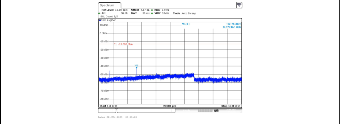
Band5-5MHz-QPSK-20625-1RB#0-Range4:1000~10000MHz
