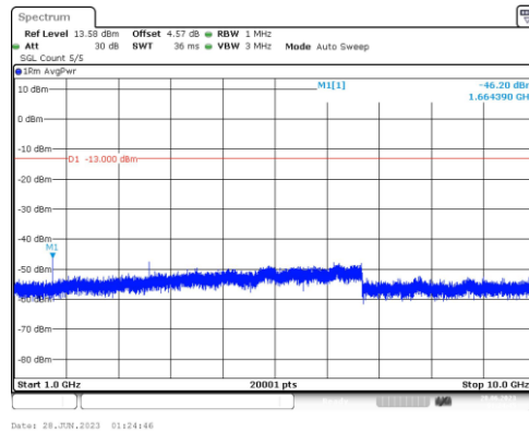
Band5-10MHz-16QAM-20525-1RB#0-Range4:1000~10000MHz
