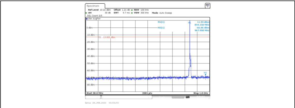
Band5-5MHz-QPSK-20625-1RB#0-Range3:30~1000MHz
