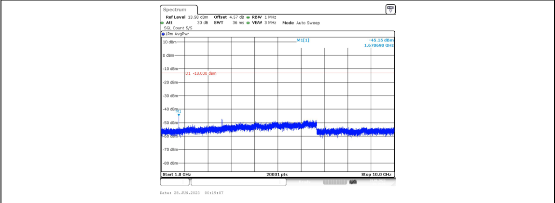
Band5-3MHz-16QAM-20525-1RB#0-Range4:1000~10000MHz
