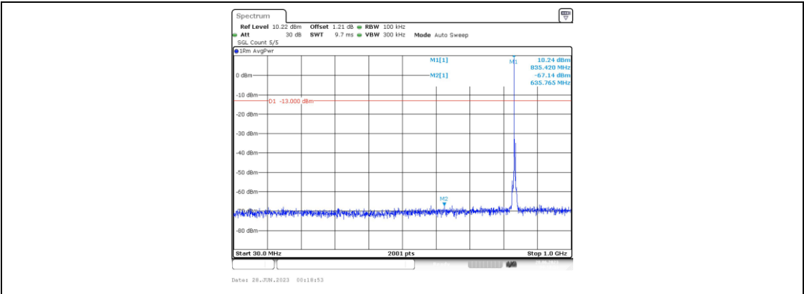
Band5-3MHz-16QAM-20525-1RB#0-Range3:30~1000MHz
