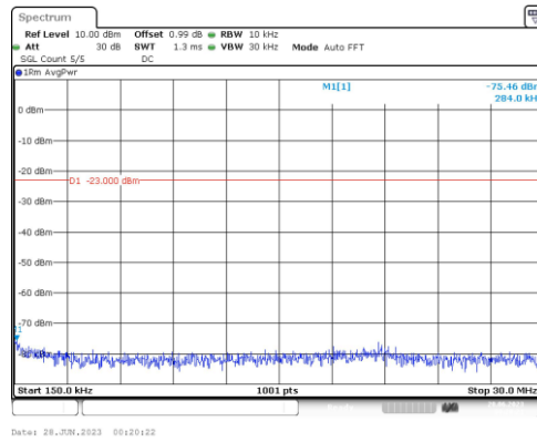
Band5-3MHz-16QAM-20635-1RB#0-Range2:0.15~30MHz
