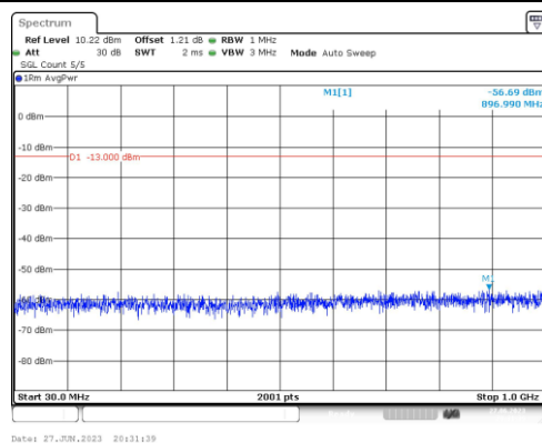
Band4-1.4MHz-16QAM-20175-1RB#0-Range3:30~1000MHz
