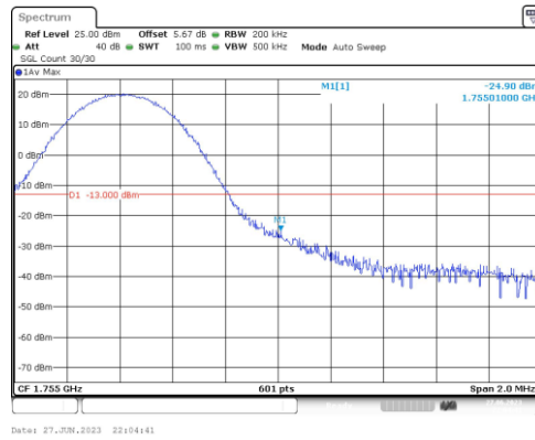
Band4-10MHz-16QAM-20350-1RB#49
