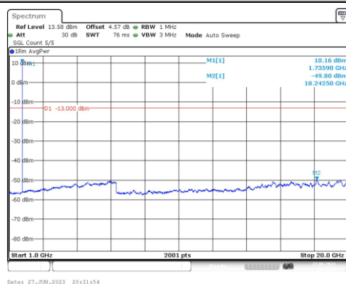
Band4-1.4MHz-16QAM-20175-1RB#0-Range4:1000~20000MHz
