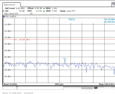
Band4-1.4MHz-QPSK-20393-1RB#0-Range1:0.009~0.15MHz
