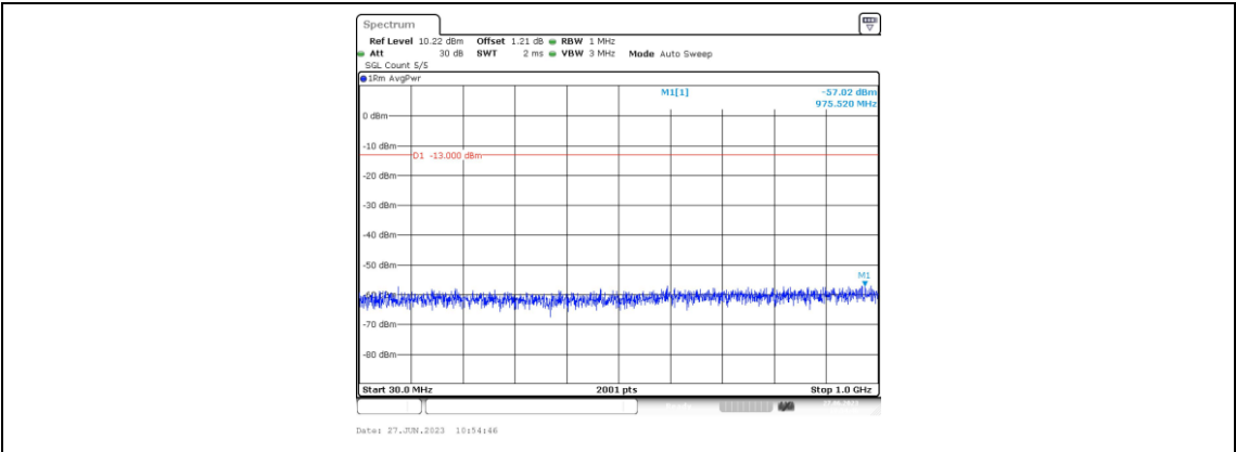
Band2-5MHz-QPSK-19175-1RB#0-Range3:30~1000MHz
