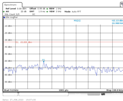
Band2-20MHz-16QAM-18700-1RB#0-Range1:0.009~0.15MHz
