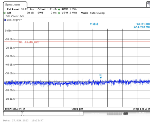
Band2-15MHz-16QAM-18900-1RB#0-Range3:30~1000MHz
