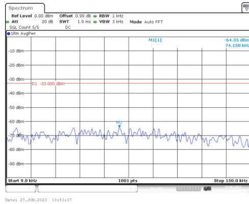
Band2-5MHz-16QAM-18900-1RB#0-Range1:0.009~0.15MHz
