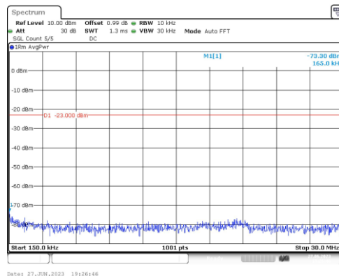
Band2-15MHz-16QAM-18900-1RB#0-Range2:0.15~30MHz
