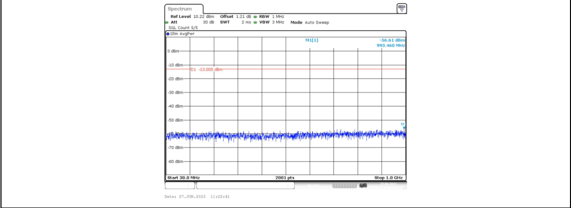
Band2-10MHz-QPSK-18650-1RB#0-Range3:30~1000MHz
