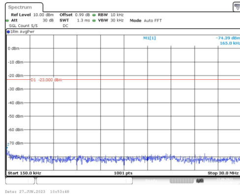
Band2-5MHz-16QAM-18900-1RB#0-Range2:0.15~30MHz
