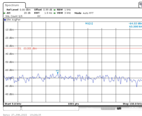
Band2-15MHz-16QAM-18900-1RB#0-Range1:0.009~0.15MHz
