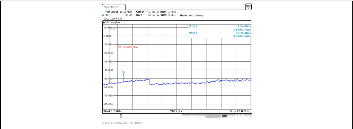
Band2-1.4MHz-QPSK-18607-1RB#0-Range4:1000~20000MHz
