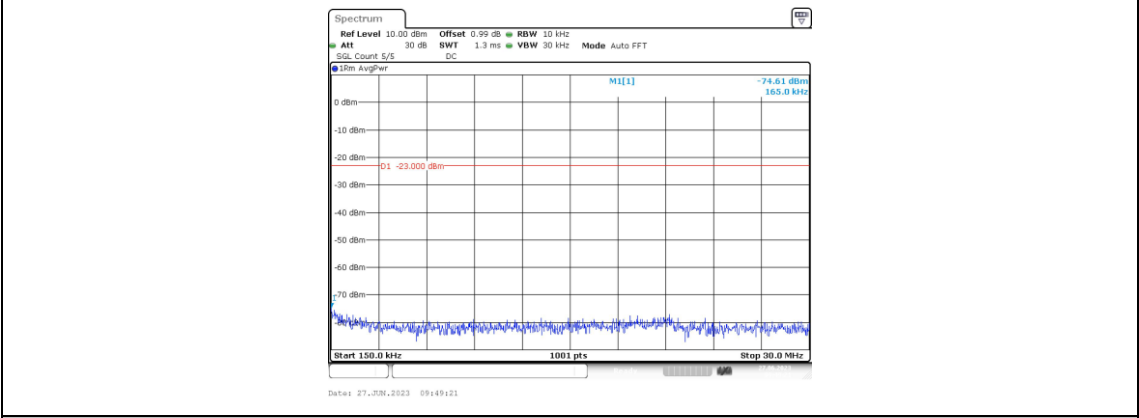
Band2-1.4MHz-16QAM-18607-1RB#0-Range2:0.15~30MHz
