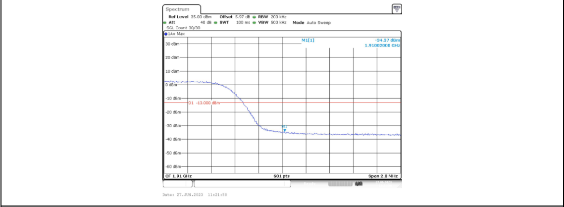
Band2-10MHz-QPSK-19150-50RB#0
