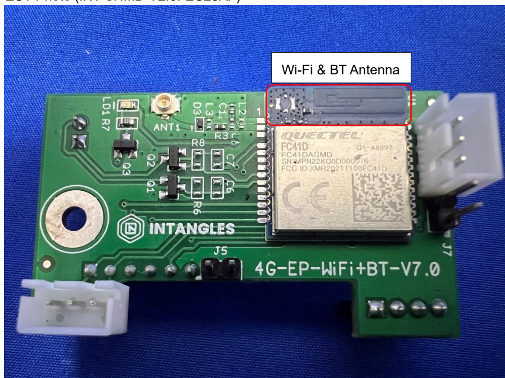
(8) EUT Photo (INT-SHMD-V2.0I-EC25AF)
