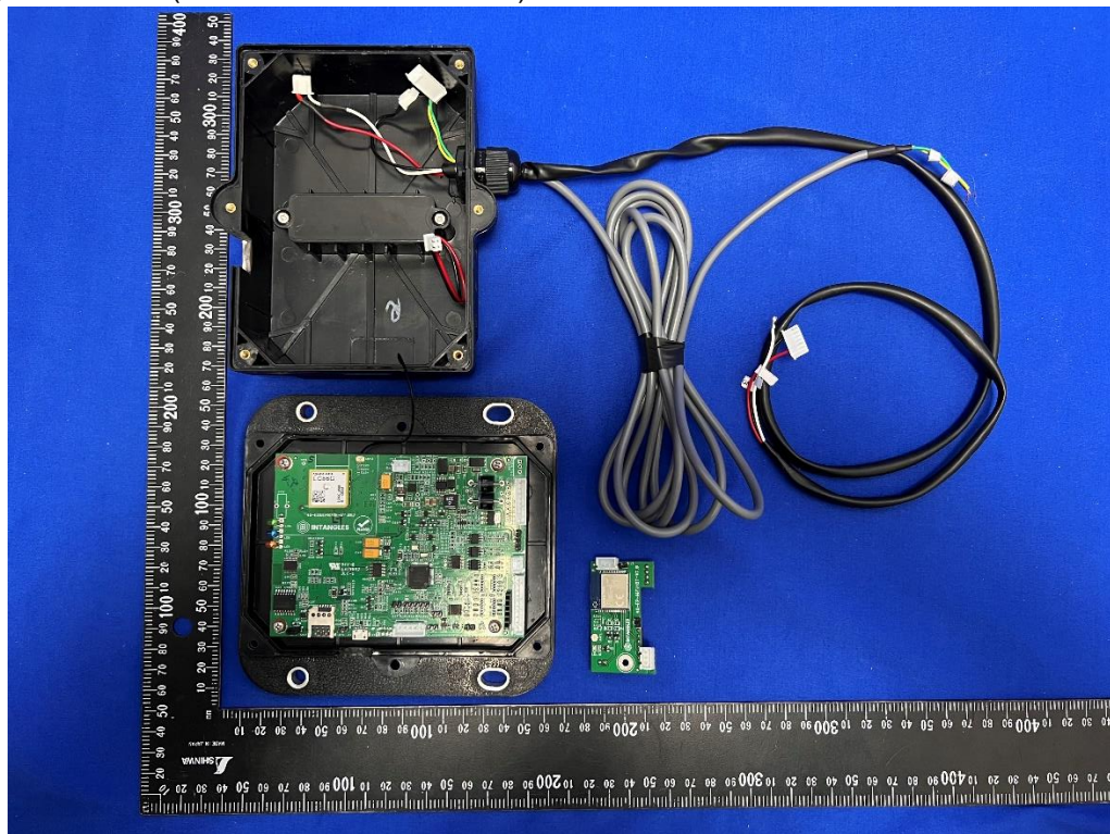
(1) EUT Photo (INT-SHMD-V2.0I-EC25AF)
