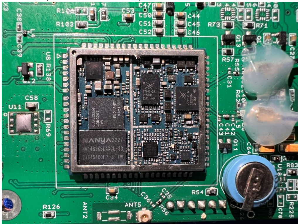
(5) EUT Photo (INT-SHMD-V2.0I-EC25AF)
