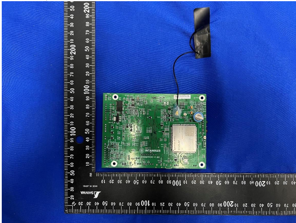
(3) EUT Photo (INT-SHMD-V2.0I-EC25AF)
