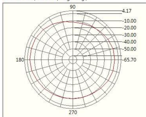
1.71GHz@Theta
