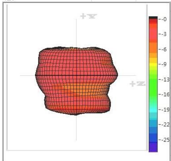
1.71GHzRight-Left
