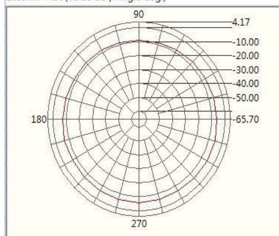
3.4GHz@Theta
