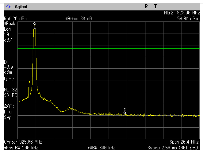
High Ch_914.9MHz_125kHz_20dBc_Upper Band Edge
