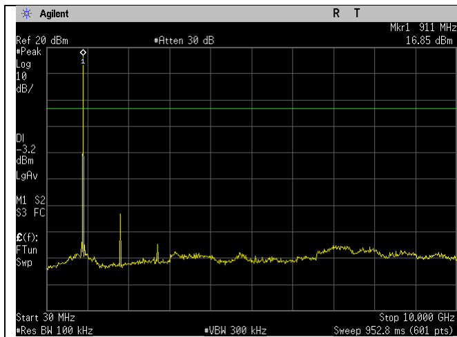
Mid Ch 908.6MHz_125kHz_20dBc_30MHz-10GHz
