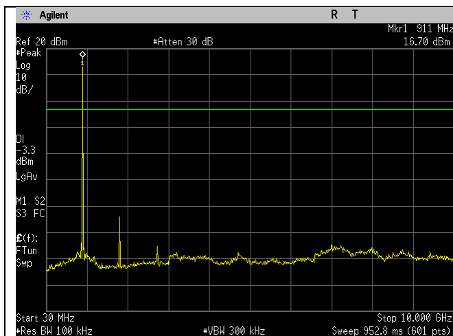
High Ch_914.9MHz_125kHz_20dBc_30MHz-10GHz
