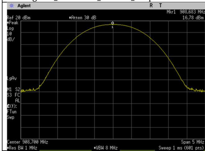
Mid Ch_908.7MHz_125kHz_Output Power
