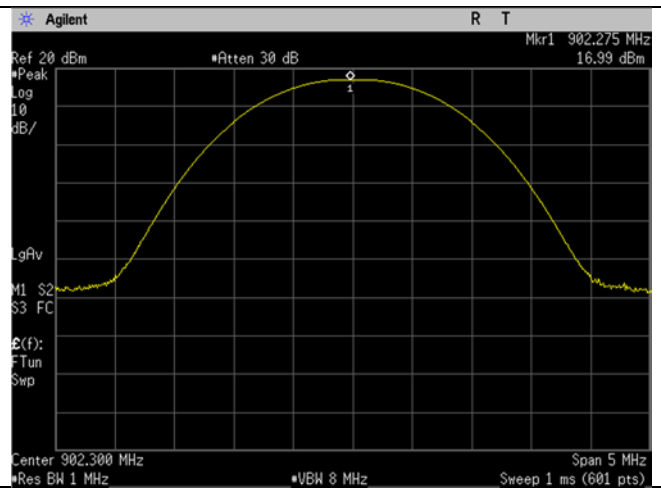
Low Ch_902.3MHz_125kHz_Output Power
