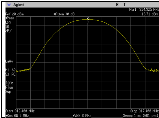
High Ch_914.9MHz_125kHz_Output Power
