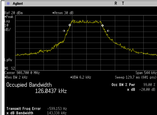
Mid Ch_908.7MHz_125kHz_Occupied Bandwidth_-20dB
