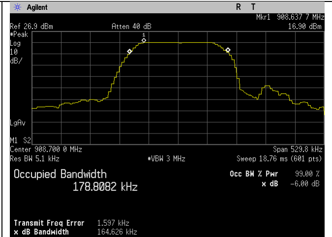
Mid Ch_908.7MHz_125kHz_Occupied Bandwidth_99 percent
