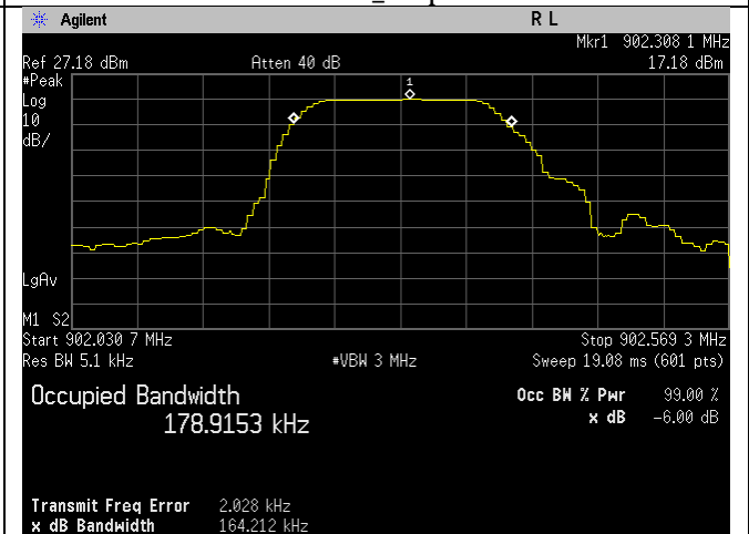
Low Ch_902.3MHz_125kHz_Occupied Bandwidth_99 percent
