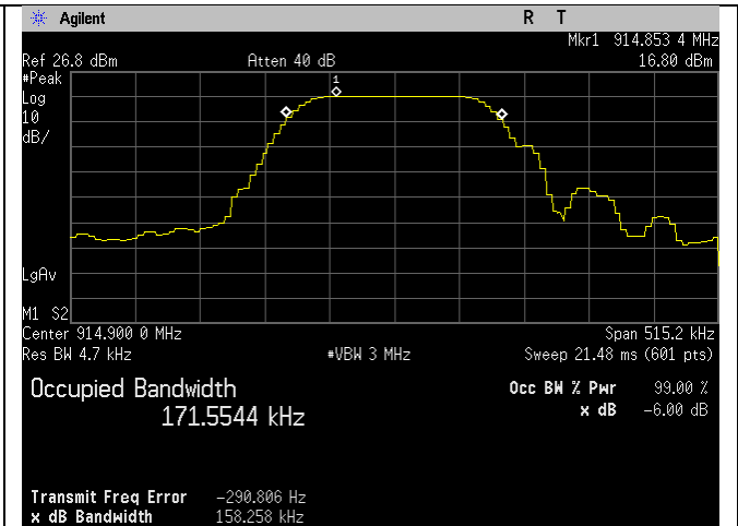
High Ch_914.9MHz_125kHz_Occupied Bandwidth_99 percent
