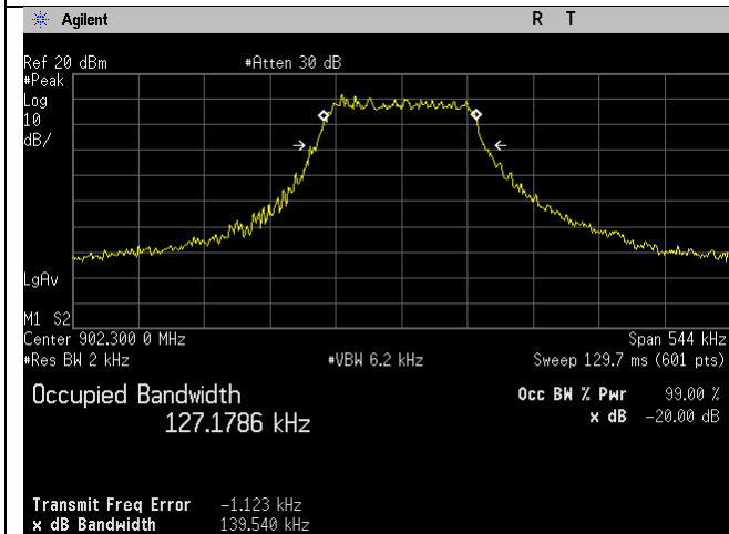
Low Ch_902.3MHz_125kHz_Occupied Bandwidth_-20dB
