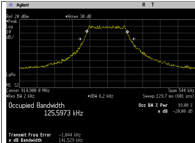
High Ch_914.9MHz_125kHz_Occupied Bandwidth_-20dB
