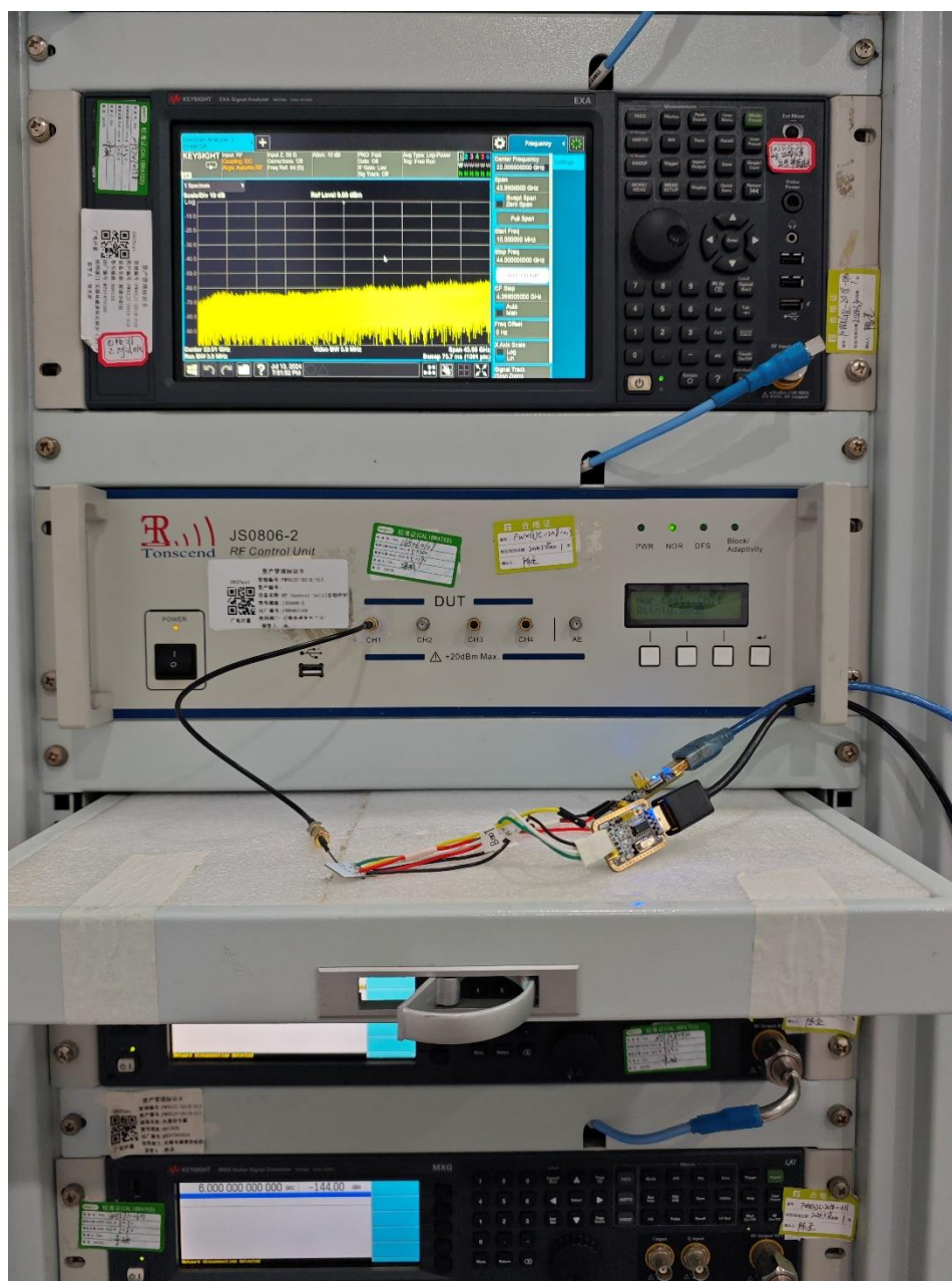
Description: Conducted Test Setup Photo
