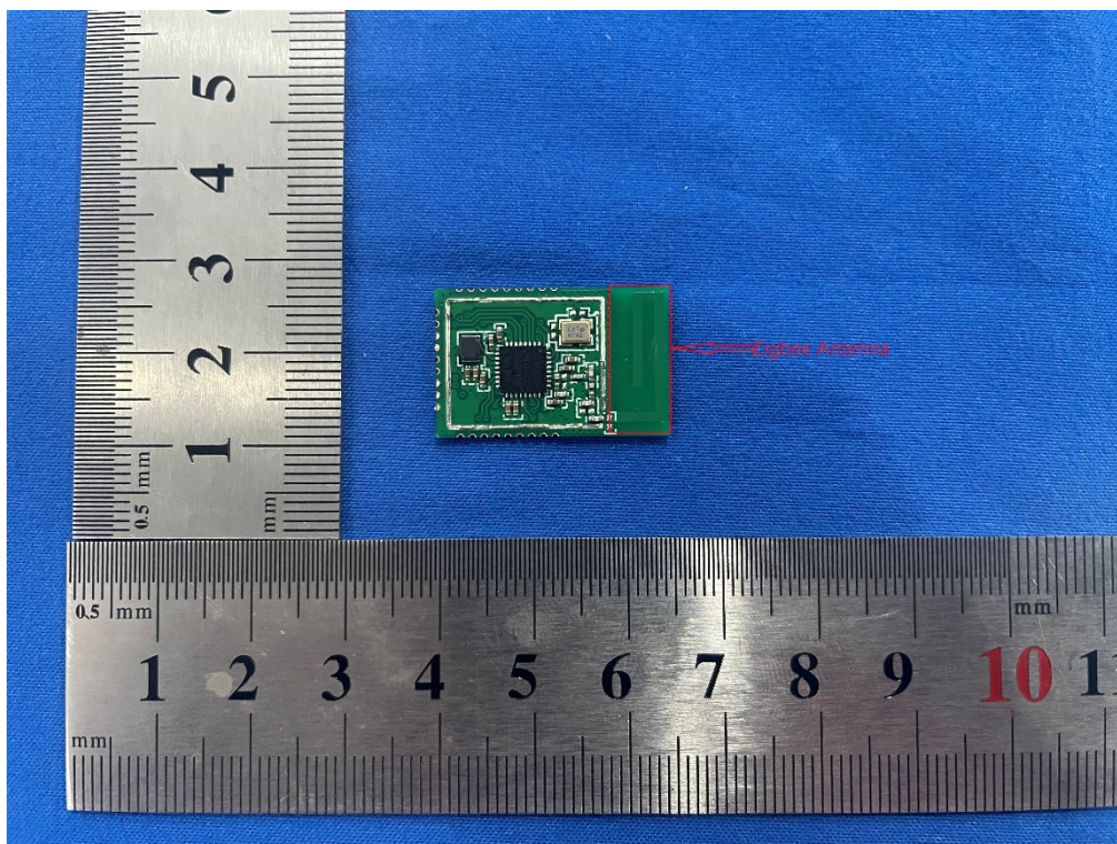
Photo 4: Internal View for Zigbee Antenna
