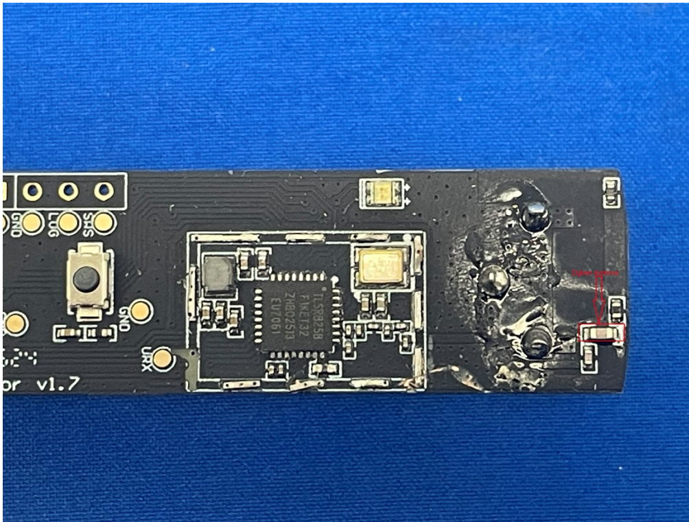
Photo 7: Internal View for Zigbee Antenna
