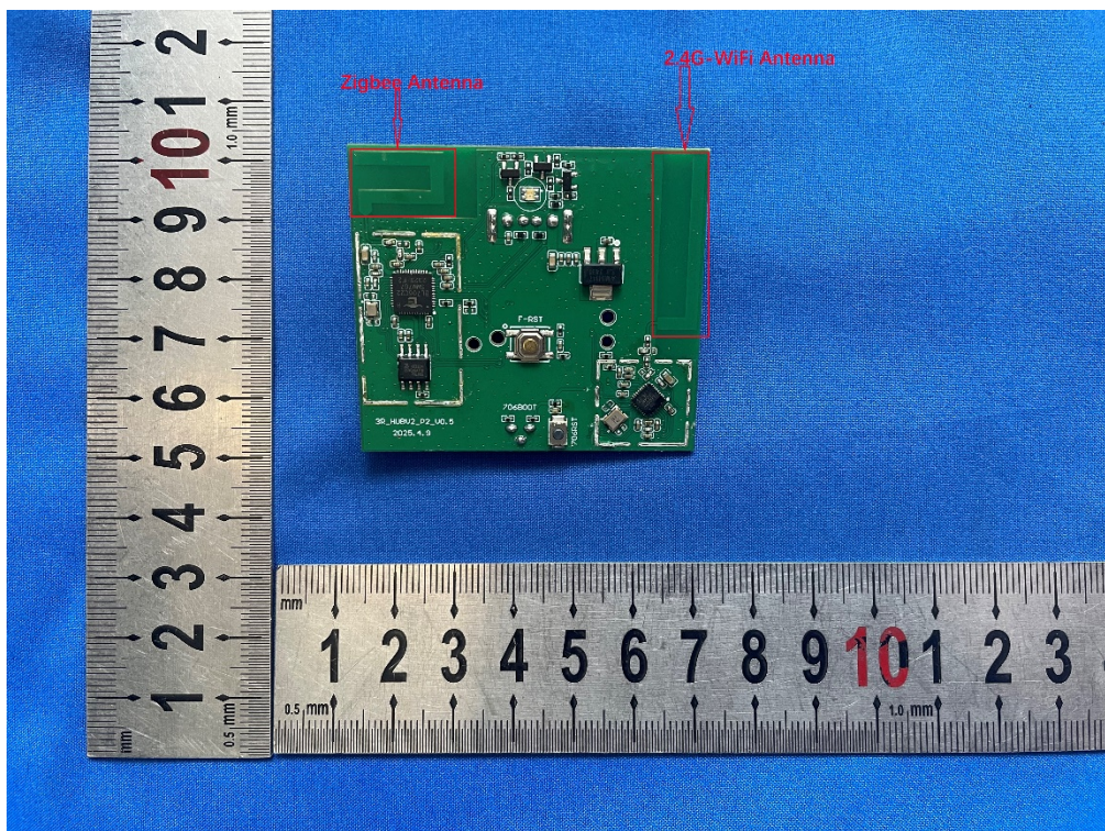
Photo 8: Internal View for Zigbee Antenna and 2.4G-WiFi Antenna
