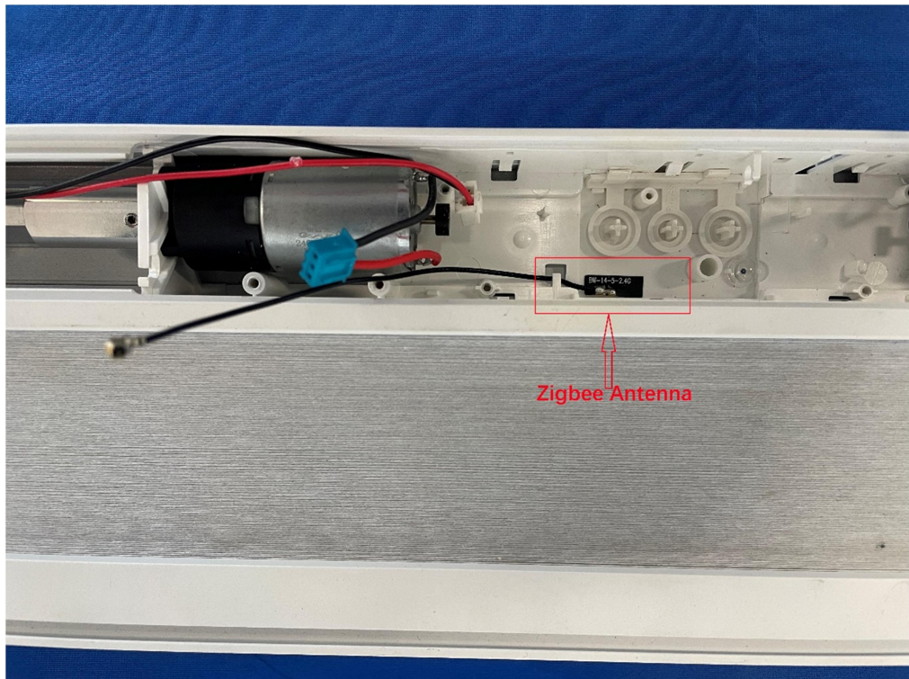
Photo 11: Internal View for Zigbee Antenna
