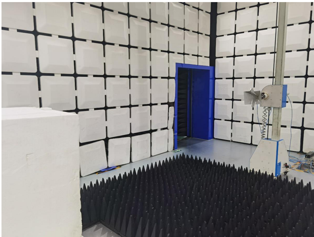
Description: Radiated Emission Test Setup for 1GHz ~ 18GHz (Mode1,2,3)
