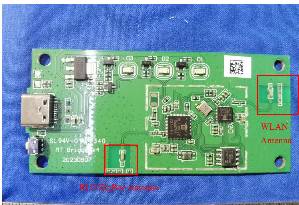
Photo 4: Antenna
