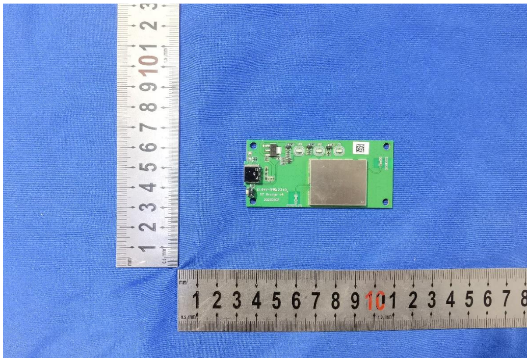
Photo 1: Internal View for PCB
