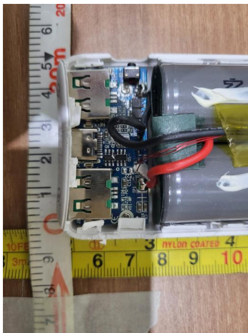
[Battery board]
